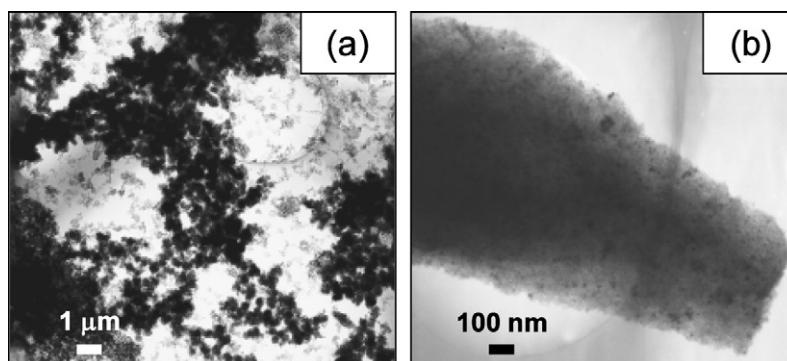
Fig. 7. TEM micrographs showing: (a) the large aggregates of \text{Fe}_2\text{O}_3 corresponding to the thick film; and (b) small \text{Fe}_2\text{O}_3 nanoparticles.
