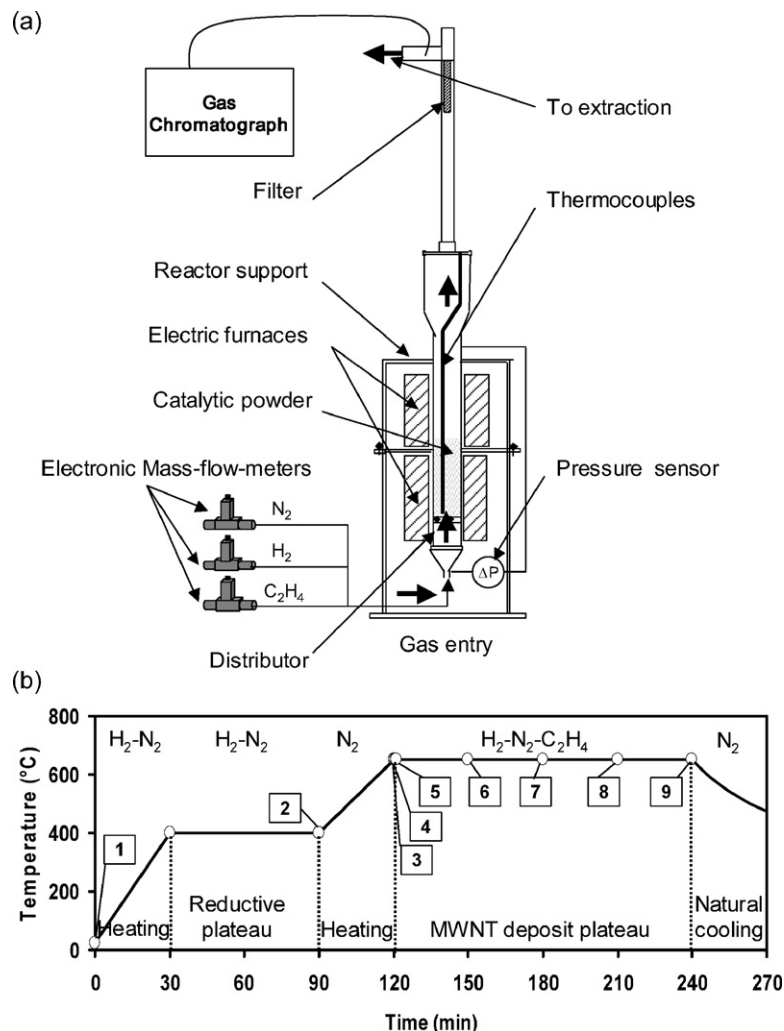
Fig. 1. (a) Experimental set-up; and (b) detailed MWCNT synthesis route and selected points for the characterizations of the catalyst.
