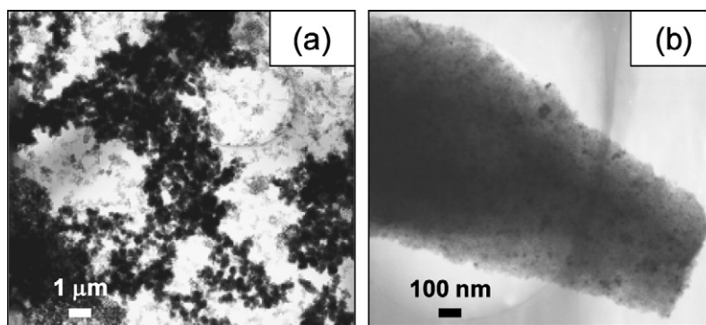
Fig. 7. TEM micrographs showing: (a) the large aggregates of Fe 2 O 3 corresponding to the thick film; and (b) small Fe 2 O 3 nanoparticles.
