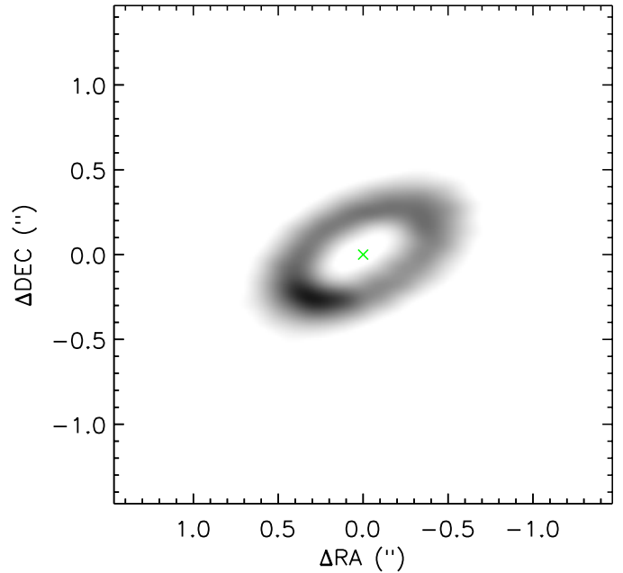
Fig. 7. ALMA band 7 continuum image (van der Plas et al. 2017). The disk is detected in as an annulus, with an azimuthal asymmetry at PA=135. Contrary to the SPHERE detection of the scattering surface, the submillimeter image probes the midplane of the disk. Therefore, the annulus detected with ALMA does not show a height-induced offset, but is centered around the star.
