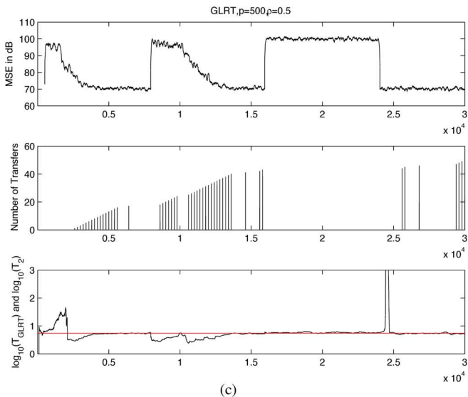
Fig. 8. GLRT-based EC performance for synthetic data. (Top) MSE. (Middle) Number of transfers from the shadow filter to the main filter. (Bottom) Time-average sufficient statistics T_{\text{GLRT}}(n) and threshold. (a) p = 100 . (b) p = 200 . (c) p = 500 .
