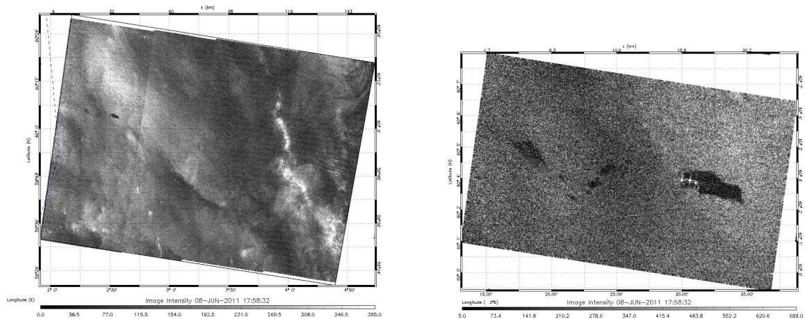
Figure 5. OOW NOFO experiment (June 2011)—Case 1 (8 June 2011, 17 h 58'): ScanSAR Wide (X band) image in VV pol. with pollution in the upper left region (left) and zoom over the detected oil spills (right).
