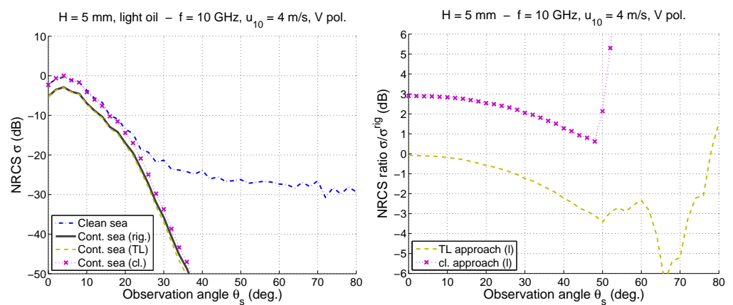
Figure 8. Monostatic NRCS \sigma (left hand-side figure) with respect to the observation angle \theta_s (deg.) according to scenario 4 described in [16] ( u_{10} = 4 m/s, V polarization, f = 10 GHz), for a light oil with thickness H = 5 mm, but with emulsified oil with equivalent relative permittivity \epsilon_{r2}^{eq} = 17 + 4i : Comparison between clean and contaminated seas with the rigorous method, and with a contaminated sea by using the two simplifying approaches. The right hand-side figure shows, for a contaminated sea, the ratio between the NRCS of the simplifying approaches and of the rigorous method for light oil.
