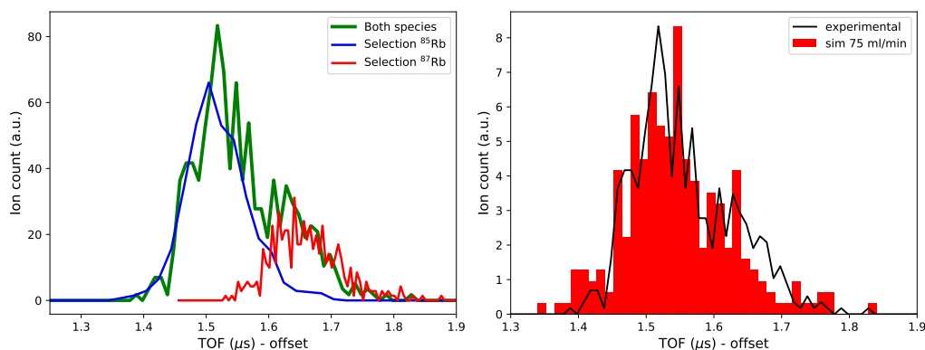
Figure 6. (Left) Time-of-flight distribution of rubidium ions behind the RFQ cb in three configurations: without any selection from the QMF (green); with QMF selecting 85 Rb + (blue); with QMF selecting 87 Rb + (red). The blue and red curves are normalized to 85,87 Rb relative abundance. (Right) Comparison of the simulated (red) TOF distribution of a 85 Rb + - 87 Rb + mixture with 75 mL/min helium flow rate to the experimentally measured one (black).
