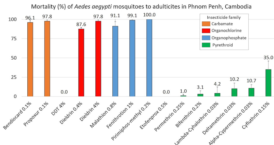
Fig. 1 Mortality (%) of adult Aedes aegypti from Phnom Penh after exposure to the selected insecticides. Error bars indicate SDs
