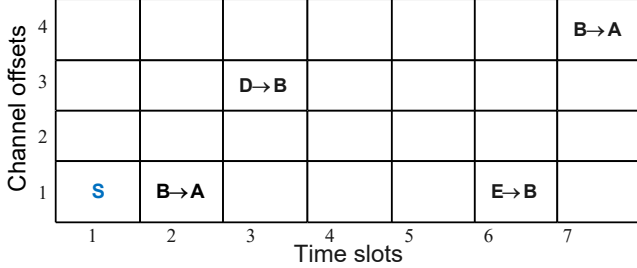
Fig. 1. Example of a TSCH schedule.
