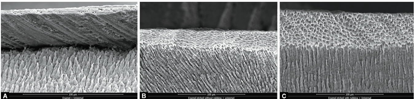
Figs 2A to C: (A) scanning electron microscope (SEM) micrographs of the enamel-adhesive interface in self-etch mode reveal a smoothie internal surface of the universal adhesive layer with no tags penetration ( \times 1,500 magnification); (B) SEM micrograph of the enamel-adhesive interface in etch-and-rinse mode showing a roughened surface due to the etching step of the enamel surface ( \times 1,500 magnification); (C) SEM image of the enamel adhesive interface in etch-and-rinse mode with rubbing technique showing a larger and greater tags penetration depth on the internal surface of the universal adhesive layer ( \times 1,500 magnification)
