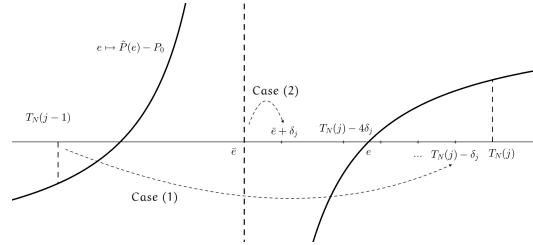
FIGURE 5. Computation of the internal energy for a mixture of two SG and a NASGK-CK liquid. Typical graph of \mathcal{P} .
