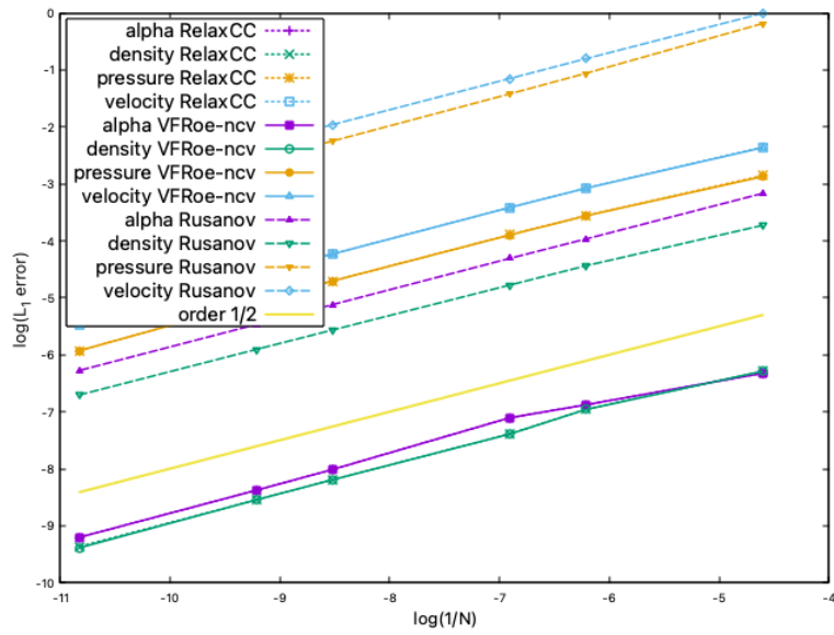
FIGURE 6. Mixture of three Stiffened Gases. L^1 -convergence for the low-pressure Riemann problem.
