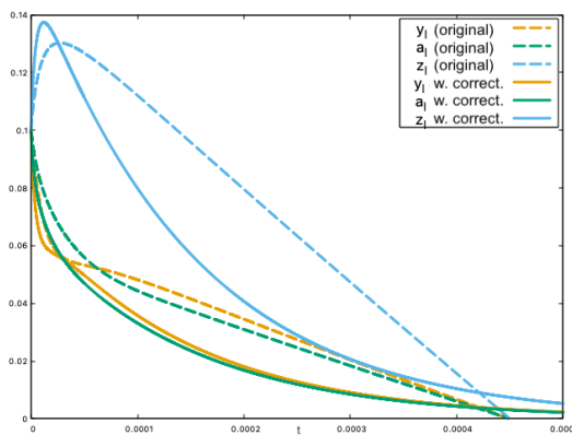
FIGURE 3. Gradient of entropy source term for a three SG mixture. Trajectories of the fractions in time without the correction (dashed lines) and with the correction (plain lines).
