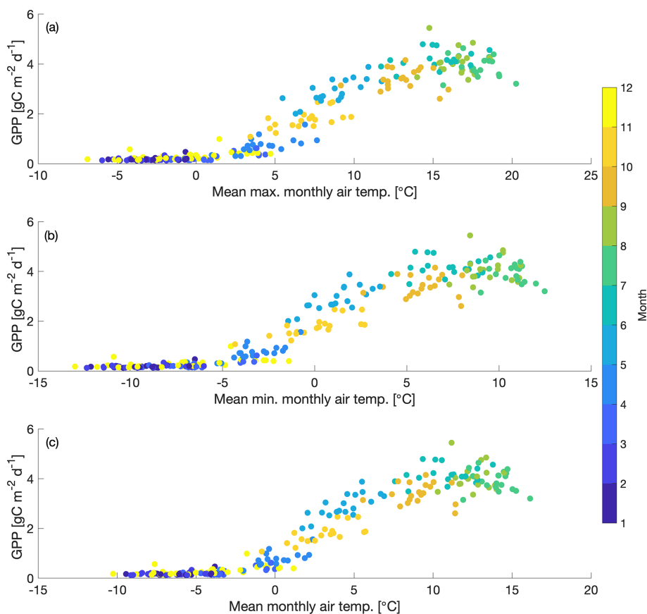
Figure 3. Scatterplot of mean monthly GPP vs. (a) mean maximum air temperature, (b) mean minimum air temperature and (c) mean air temperature for 2000–2018. Dots are colored with the corresponding month.
