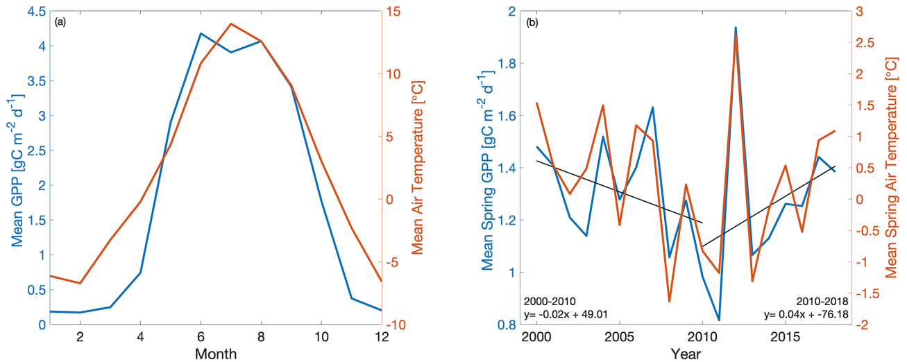
Figure 1. Time series of (a) mean monthly GPP (blue) and air temperature (orange) and (b) mean spring (March–May) GPP and air temperature at Niwot Ridge (US-NR1) from 2000–2018. GPP data are derived using a nighttime partitioning technique based on tower observations of NEE and air temperature.
