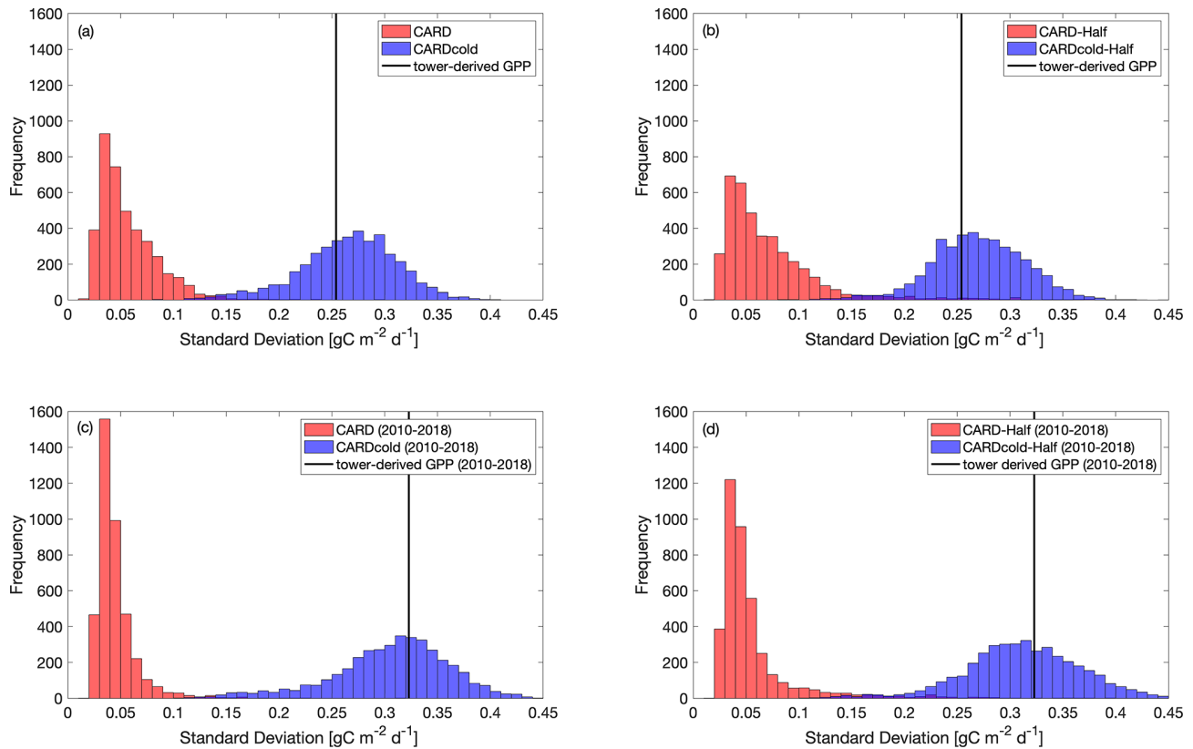
Figure 6. Histograms comparing standard deviation in mean spring GPP across all ensembles ( N = 4000 ) for CARD (red bars) and CARD-cold (blue bars) experiments with (a) full assimilation, (b) half assimilation, (c) full assimilation for the second decade (2010–2018) and (d) half assimilation for the second decade (2010–2018). The black line indicates the standard deviation in tower-derived mean spring GPP (SD = 0.25 \text{ g C m}^{-2} \text{ d}^{-1} for full period (a–b); SD = 0.32 \text{ g C m}^{-2} \text{ d}^{-1} for 2010–2018 (c–d)).
