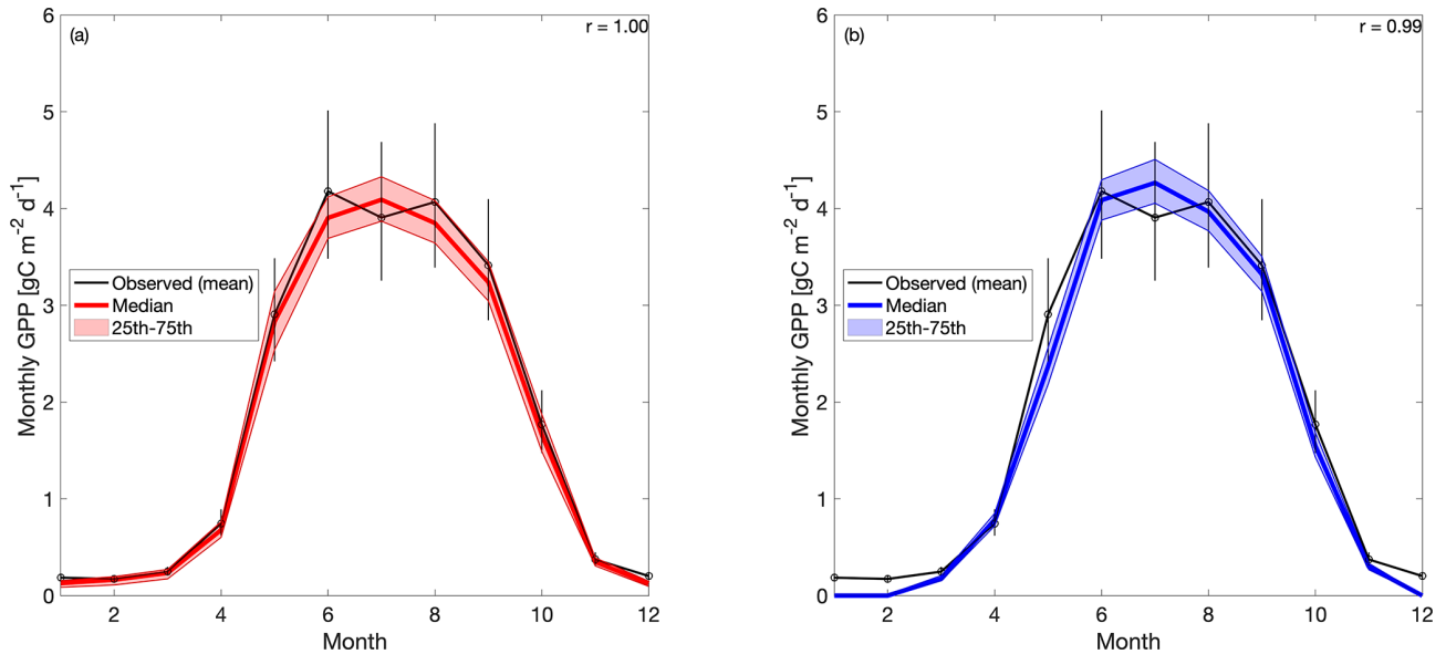
Figure 4. Tower-derived average monthly GPP (black line) and modeled GPP seasonal cycles at US-NR1 for 2000–2018, for (a) CARD and (b) CARDcold experiments. The half-assimilation experiments (CARD-Half and CARDcold-Half) can be found in the Supplement (Fig. S5). Model outputs include the median value of each experiment (bold colored line) with the 25th–75th percentiles of the ensembles (shaded area). The median is plotted instead of the mean to avoid impact of outlier ensemble members ( N = 4000 ). Error bars are tower-derived GPP multiplied and/or divided by \exp(\sqrt{(\log(2))^2 \cdot n}/n) . n is number of years on average ( n = 19 ). r is Pearson's coefficient.
