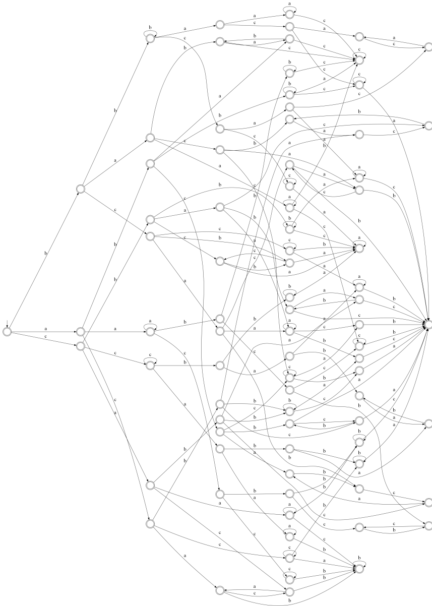
Figure 7. A DFA recognizing 2-abelian singletons over \{a, b, c\} .
