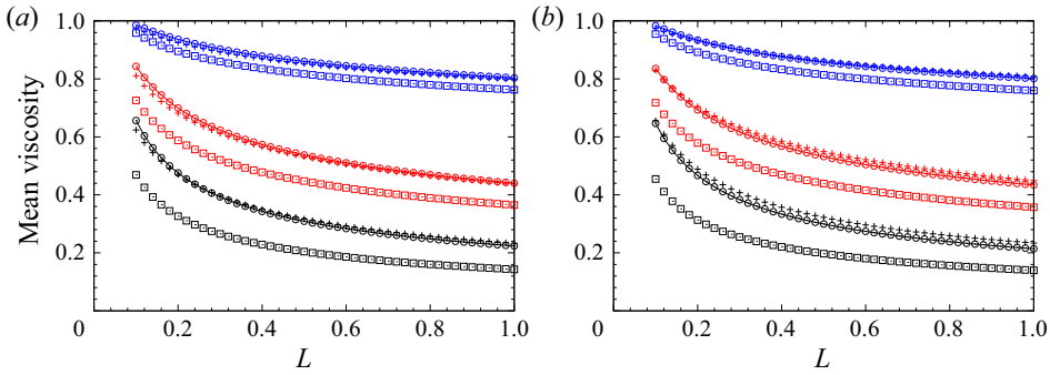
Figure 26. Average and equivalent viscosities for the convective flow at the saddle-node points SN_1 (a) and SN_2 (b) in a shear-thinning fluid. Here, \circ : equivalent viscosity; \square : Parmentier's viscosity; + : bulk-average viscosity. These viscosities are given as a function of L for three values of the power-law index n : 0.9 (blue), 0.7 (red) and 0.5 (black).
