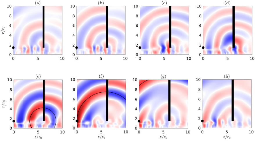
Figure 16: Correlations \mathcal{R} of p'(r = 1.5r_0, z = 0, t) with p'(r, z, t + \delta t) for n_\theta = 1 for (a) \delta t = -15r_0/u_j , (b) \delta t = -12r_0/u_j , (c) \delta t = -9r_0/u_j , (d) \delta t = -6r_0/u_j , (e) \delta t = -3r_0/u_j , (f) \delta t = 0 , (g) \delta t = 3r_0/u_j and (h) \delta t = 6r_0/u_j for jetmediumhole; — circle centered on (z = L, r = 1.5r_0) . The color scale ranges between \pm 1 , from blue to red.
