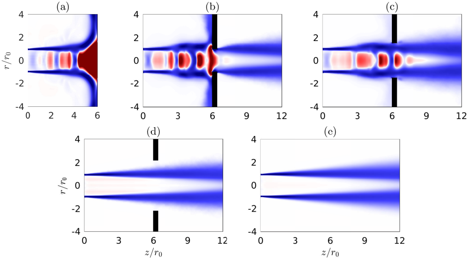
Figure 5: Mean density fields in the (z, r) plane for (a) jetnohole, (b) jetsmallhole, (c) jetmediumhole, (d) jetlargehole and (e) the free jet. The color scale ranges from 0.95\rho_0 up to 1.05\rho_0 , from blue to red.
