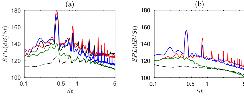
Figure 12: Sound pressure levels (SPL) at (a) z = 0 and r = 1.5r_0 and (b) z = 12r_0 and r = 15r_0 as a function of the Strouhal number St = fD/u_j ; — jetnohole, — jetsmallhole, — jetmediumhole, — jetlargehole and - - - free jet.
