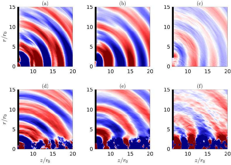
Figure 26: Pressure fields obtained downstream of the plate (top) using equation (3.4) and (bottom) from LES for (a,d) jetsmallhole, (b,e) jetmediumhole and (c,f) jetlargehole. The color scales range between (a,b,d,e) \pm 0.01p_0 , and (c,f) \pm 0.0025p_0 , from blue to red.
