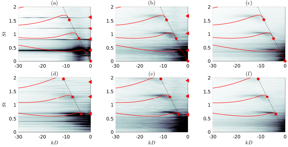
Figure 20: Frequency-wavenumber spectra of the pressure fluctuations at r = r_0 for (a,d) jetmediumhole, (b,e) jetlargehole and (c,f) the free jet for (top) n_\theta = 0 and (bottom) n_\theta = 1 ; — dispersion curves and * lower limits of the guided jet modes for a vortex-sheet model, ◀ LES tone frequencies and - - k = -\omega/c_0 . The greyscale levels spread over 25 dB.
