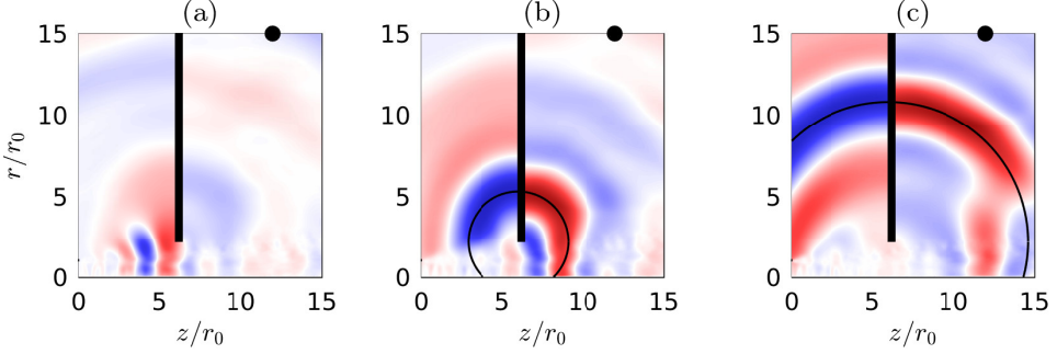
Figure 19: Correlations \mathcal{R} of p'(r = 15r_0, z = 12r_0, t) with p'(r, z, t + \delta t) for n_\theta = 1 for (a) \delta t = -15r_0/u_j , (b) \delta t = -10r_0/u_j and (c) \delta t = -5r_0/u_j for jetlargehole; — circle centered on (z = L, r = 2.2r_0) . The color scale ranges between \pm 1 , from blue to red.
