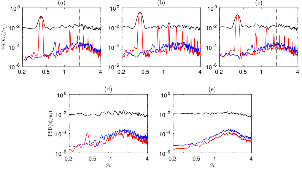
Figure 9: Power spectral densities of radial velocity fluctuations u'_r obtained at r = r_0 and z = 0.4r_0 for (a) jetnohole, (b) jetsmallhole, (c) jetmediumhole, (d) jetlargehole and (e) the free jet; — full signal, — n_\theta = 0 and — n_\theta = 1 , - - St_\theta = f\delta_\theta/u_j = 0.016 .
