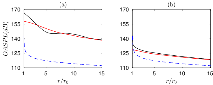
Figure 25: Overall sound pressure levels obtained at z = 0 — from LES and — using equation (3.4), for (a) jetsmallhole and (b) jetlargehole, - - - levels for jetfree.
