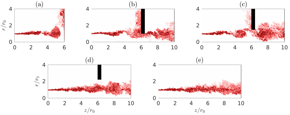
Figure 3: Snapshots in the (z, r) plane of the vorticity norm for (a) jetnohole, (b) jetsmallhole, (c) jetmediumhole, (d) jetlargehole and (e) the free jet. The color scales range from 0 up to 15u_j/r_0 , from white to red.
