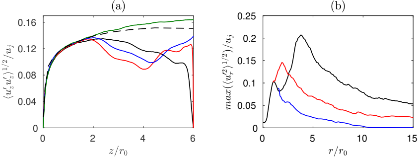
Figure 8: Variations of (a) axial turbulence intensity \langle u'_z u'_z \rangle^{1/2} / u_j at r = r_0 and (b) maximal radial turbulence intensity \langle u'_r u'_r \rangle^{1/2} / u_j in the wall jet: — jetnohole, — jetsmallhole, — jetmediumhole, — jetlargehole and - - free jet.
