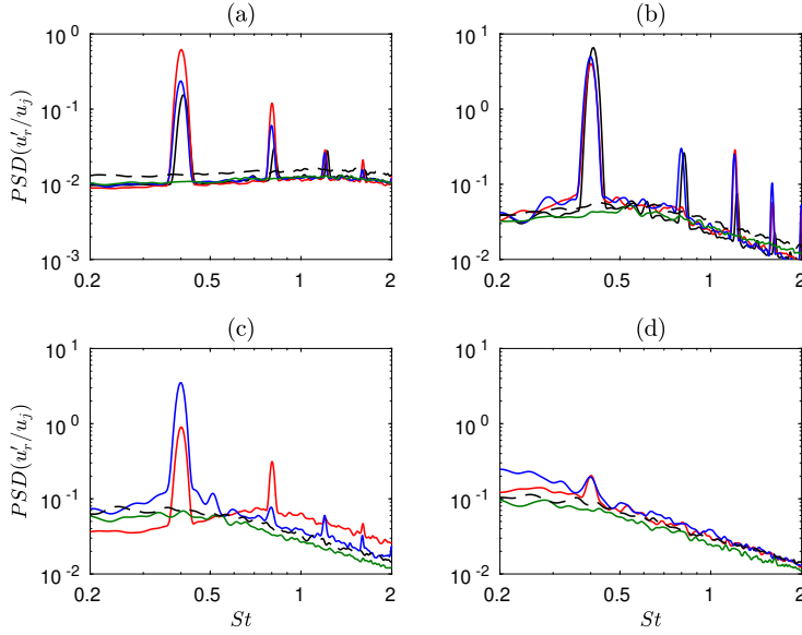
Figure 10: Power spectral densities of radial velocity fluctuations u'_r obtained at r = r_0 and (a) z = r_0 , (b) z = 5r_0 , (c) z = 7r_0 and (d) z = 12r_0 for — jetnohole, — jetsmallhole, — jetmediumhole, — jetlargehole and - - - the free jet.
