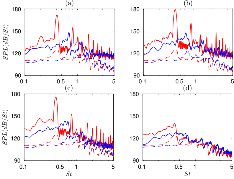
Figure 13: Sound pressure levels (SPL) at z = 0 and r = 1.5r_0 for (a) jetnohole, (b) jetsmallhole, (c) jetmediumhole and (d) jetlargehole for the azimuthal modes n_\theta = 0 and n_\theta = 1 ; SPL for n_\theta = 0 and n_\theta = 1 for the free jet.
