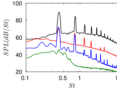
Figure 22: Pressure spectra on the plate at z = L and r = 3r_0 for — jetnohole, — jetsmallhole, — jetmediumhole and — jetlargehole.
