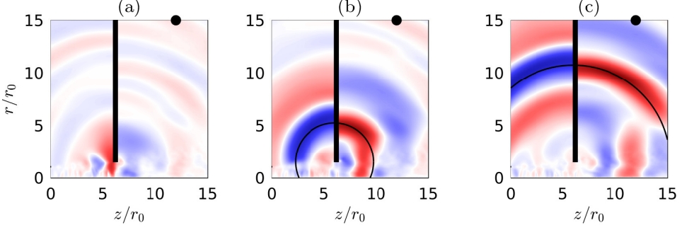
Figure 18: Correlations \mathcal{R} of p'(r = 15r_0, z = 12r_0, t) with p'(r, z, t + \delta t) for n_\theta = 1 for (a) \delta t = -15r_0/u_j , (b) \delta t = -10r_0/u_j and (c) \delta t = -5r_0/u_j for jetmediumhole; — circle centered on (z = L, r = 1.5r_0) . The color scale ranges between \pm 1 , from blue to red.
