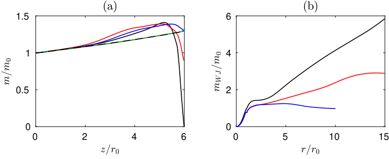
Figure 6: Variations of (a) the jet mass flow rate m in the axial direction and (b) the mass flow rate of the wall jet m_{WJ} in the radial direction for — jetnohole, — jetsmallhole, — jetmediumhole, — jetlargehole and - - - the free jet (Bogey (2018)).
