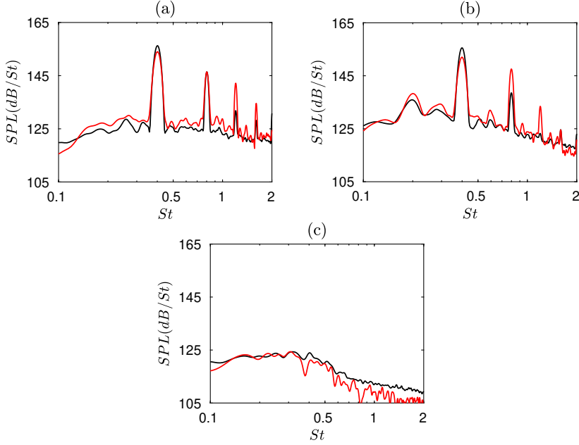
Figure 27: Sound pressure levels obtained at z = 12r_0 and r = 15r_0 from — LES and — using equation (3.4) for (a) jetsmallhole, (b) jetmediumhole and (c) jetlargehole, as a function of the Strouhal number.
