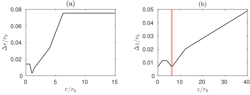
Figure 2: Variations of (a) radial and (b) axial mesh spacings; — positions of the upstream and downstream faces of the plate.
