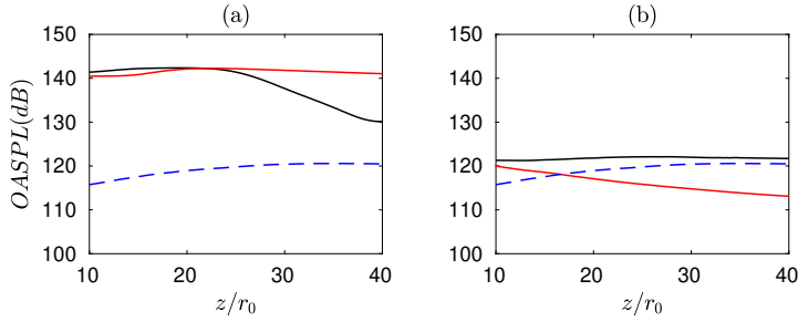
Figure 28: Overall sound pressure levels obtained downstream of the plate at r = 15r_0 — from LES and — using equation (3.4), for (a) jetsmallhole and (b) jetlargehole, - - - levels for jetfree.
