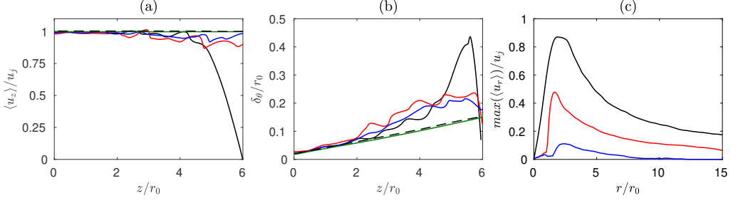
Figure 7: Variations of (a) mean axial velocity \langle u_z \rangle / u_j at r = 0 , and (b) shear-layer momentum thickness \delta_\theta / r_0 in the axial direction and of (c) the maximum mean radial velocity \langle u_r \rangle in the wall jet: — jetnohole, — jetsmallhole, — jetmediumhole, — jetlargehole and - - free jet (Bogey (2018)).
