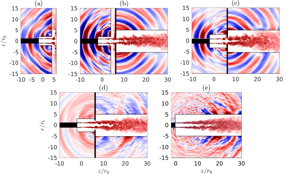
Figure 4: Snapshots in the (z, r) plane of the vorticity norm in the flow and of the fluctuating pressure outside for (a) jetnohole, (b) jetsmallhole, (c) jetmediumhole, (d) jetlargehole and (e) the free jet. The color scales range from 0 up to 7u_j/r_0 for the vorticity norm, from white to red, and between (a-c) \pm 0.01p_0 , (d) \pm 0.0025p_0 and (e) \pm 0.001p_0 for the pressure, from blue to red.
