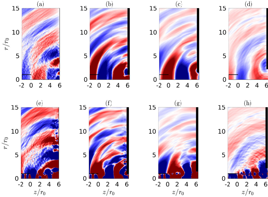
Figure 23: Pressure fields obtained upstream of the plate (top) using equation (3.4) and (bottom) from LES for (a,e) jetnohole, (b,f) jetsmallhole, (c,g) jetmediumhole and (d,h) jetlargehole. The color scales range between (a,b,c,e,f,g) \pm 0.01p_0 , and (d,h) \pm 0.0025p_0 , from blue to red.
