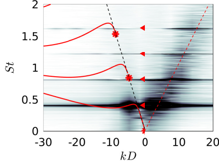
Figure 21: Frequency-wavenumber spectrum of the pressure fluctuations at r = r_0 for jetmediumhole for n_\theta = 0 ; — dispersion curves and * lower limits of the guided jet modes for a vortex-sheet model, ◄ LES tone frequencies, - - - k = -\omega/c_0 and - - - k = \omega/u_c . The greyscale levels spread over 25 dB.
