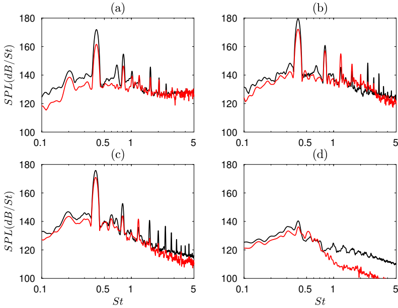
Figure 24: Sound pressure levels obtained at z = 0 and r = 1.5r_0 — from LES and — using equation (3.4), for (a) jetnohole, (b) jetsmallhole, (c) jetmediumhole and (d) jetlargehole, as a function of the Strouhal number.
