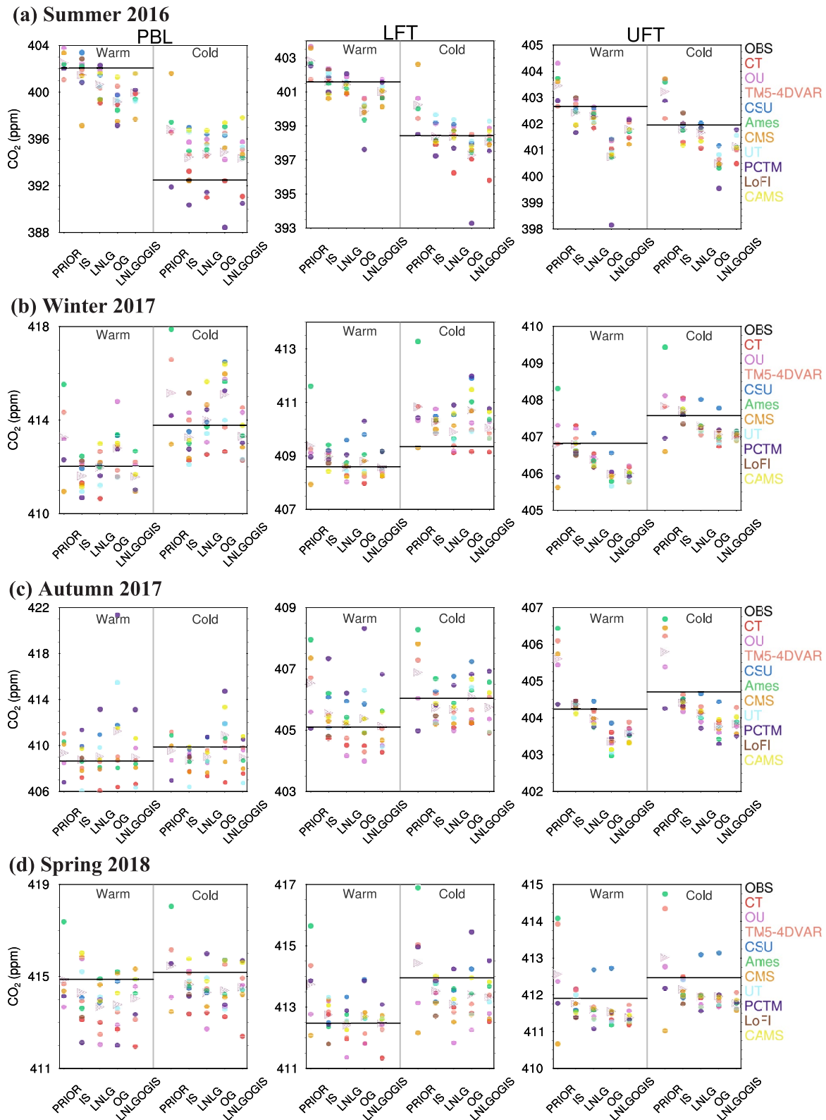
Figure 5. Mean [CO_2] in cold and warm sectors of frontal systems within the planetary boundary layer (PBL), lower free-troposphere (LFT), and upper free-troposphere (UFT) as observed with aircraft (black lines) and simulated with OCO-2 MIP members (colored dots) in five experiments (PRIOR, IS, LNLG, OG, and LNLGOGIS) in (a) summer 2016, (b) winter 2017, (c) autumn 2017, and (d) spring 2018. The triangles denote the ensemble mean of OCO-2 MIP models.
