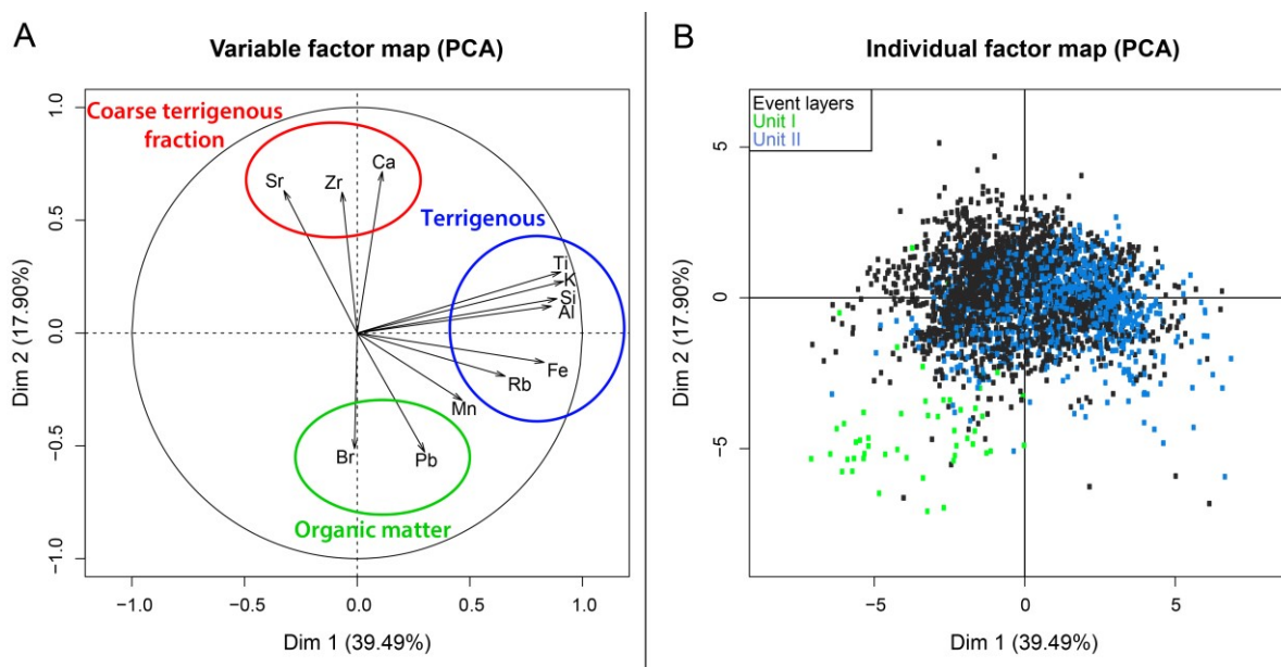
Figure 3 - Variable and individual factor maps from the principal component analysis (PCA). (A) Variable factor map with three end-members (terrigenous, organic matter and coarse terrigenous fraction linked to carbonates). (B) Individual factor map with the two sedimentological units added as an illustrative variable and compared with the event layers.
