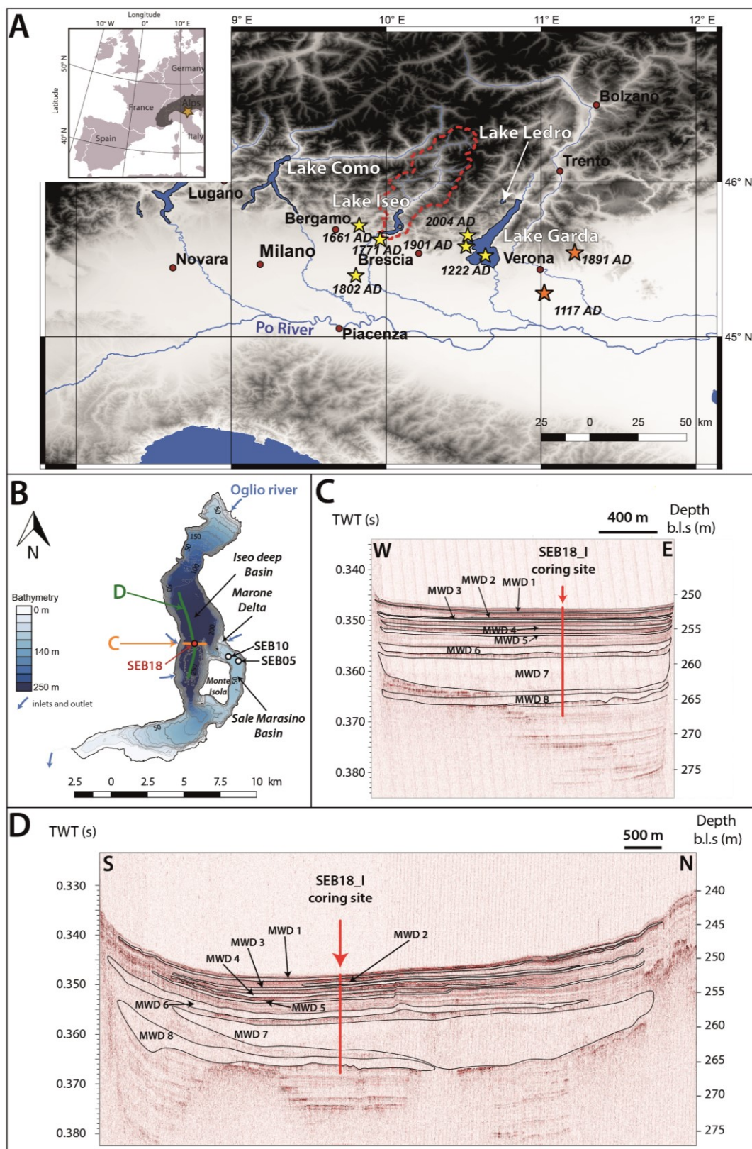
Figure 1 - Lake Iseo location and settings. (A) Location of Lake Iseo (Italy), its watershed (red dashed line) and different lakes of the Italian southern Alps: Lake Como, Lake Garda, and Lake Ledro. The orange and yellow stars correspond to the location of historic earthquakes with a Magnitude \geq 6 and < 6 , respectively. (B) Lake Iseo Bathymetric map associated with the description of the different morphological features and the different coring sites. Seismic profiles west-east (C) and south-north (D) oriented across the deep basin showing the coring site location (vertical red line) and the principal generations of mass wasting deposits (MWD, coloured lines). The depth of the seismic profile is expressed in metres below lake surface (m b.l.s.), assuming a mean P-wave velocity of 1450 m.s -1 in water and sediments.
