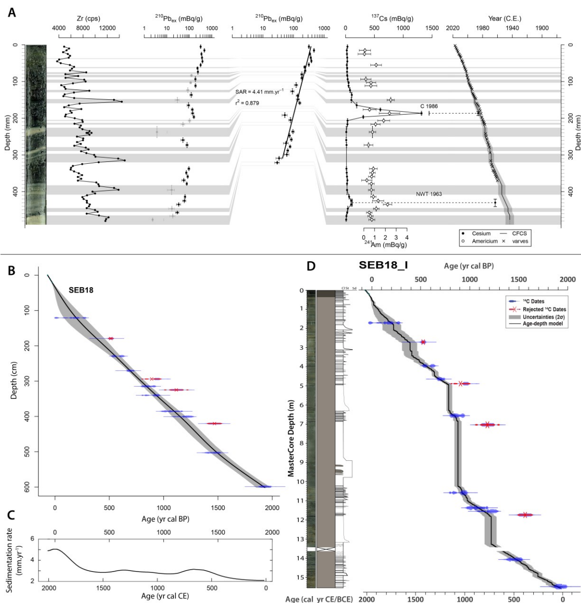
Figure 4 - Age-depth models. (A) Short-lived radionuclide data: ^{210}\text{Pb}_{\text{ex}} in logarithmic scale associated with the ^{241}\text{Am} and ^{137}\text{Cs} profiles with the picture of the top 48 cm of SEB18 sequence. (B) Age-depth model in event-free depth. (C) Sedimentation rate (without event layers) obtained from the age-depth model, (D) Complete age-depth model associating radiocarbon and varve counting.
