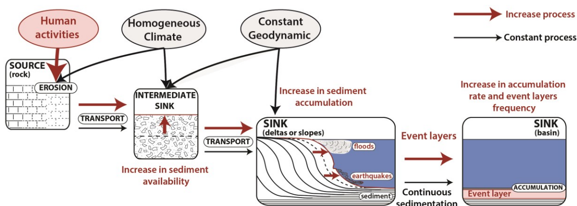
Figure 8 - Conceptual model of the erosion cycle in a large catchment and the effects of the three main forcing factors (human activities, climate and geodynamic). Modified from Rapuc et al. (2021b).
