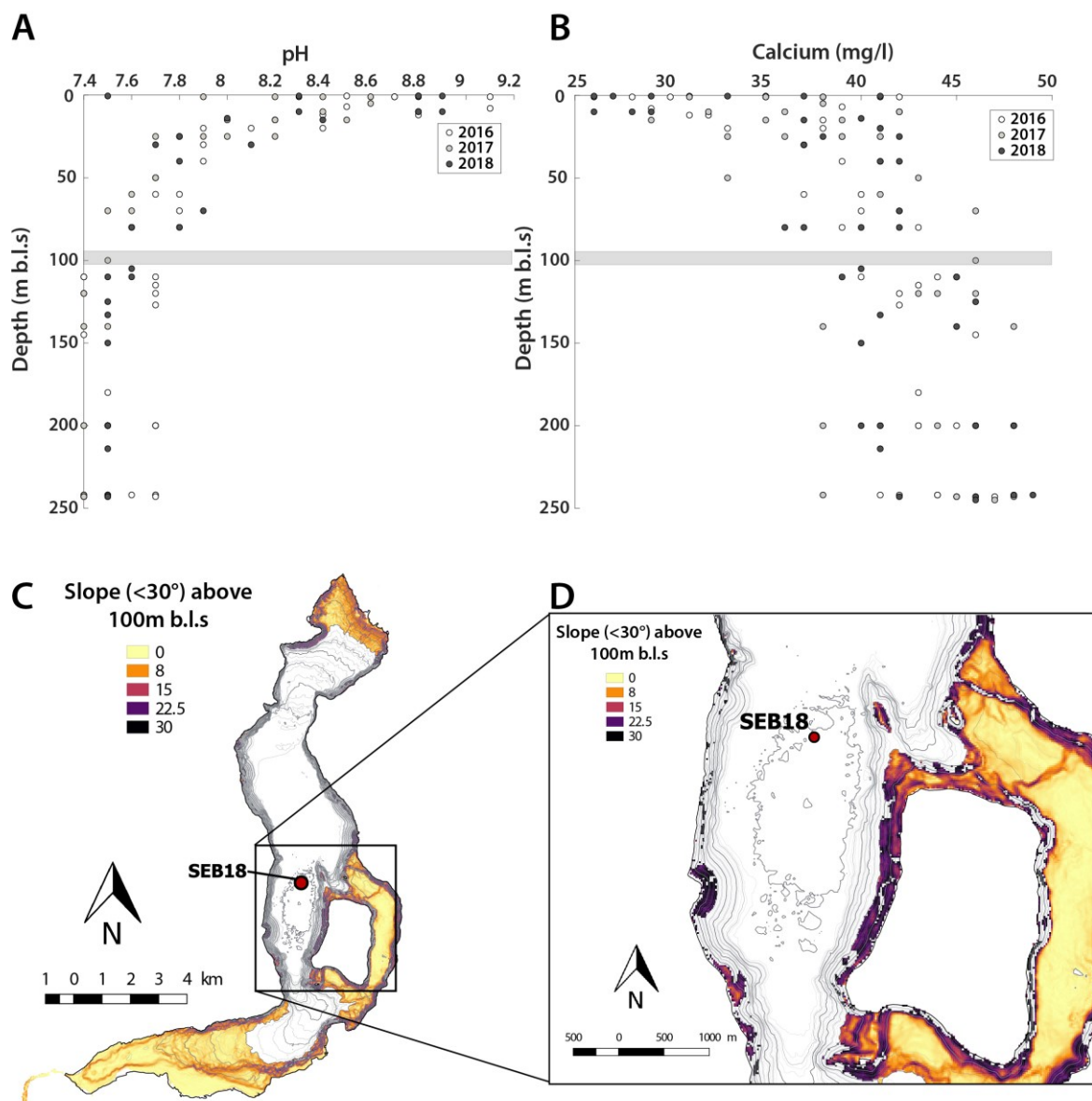
Figure 5 - pH (A) and dissolved calcium (B) profiles, recorded in the deep basin of Lake Iseo, close to the coring site, in 2016, 2017 and 2018 by ARPA ( http://arpalombardia.it/ ). (C) Map presenting slopes of Lake Iseo with an inclination lower than 30^\circ above 100 m b.l.s. where authigenic carbonates could accumulate (D) Close-up of map (C) in the deep basin around the coring site.
