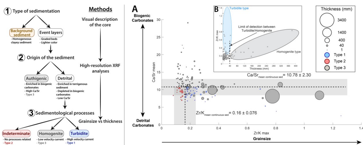
Figure 6 - (A) Scatter plot of Ca/Sr_{mean} versus Zr/K_{max} with the thickness indicate by dot sizes of each event layers. (B) Scatter plot of Zr/K_{max} values versus the thickness of each event layers. Explanation of the methodological approach is synthesized on the left panel.
