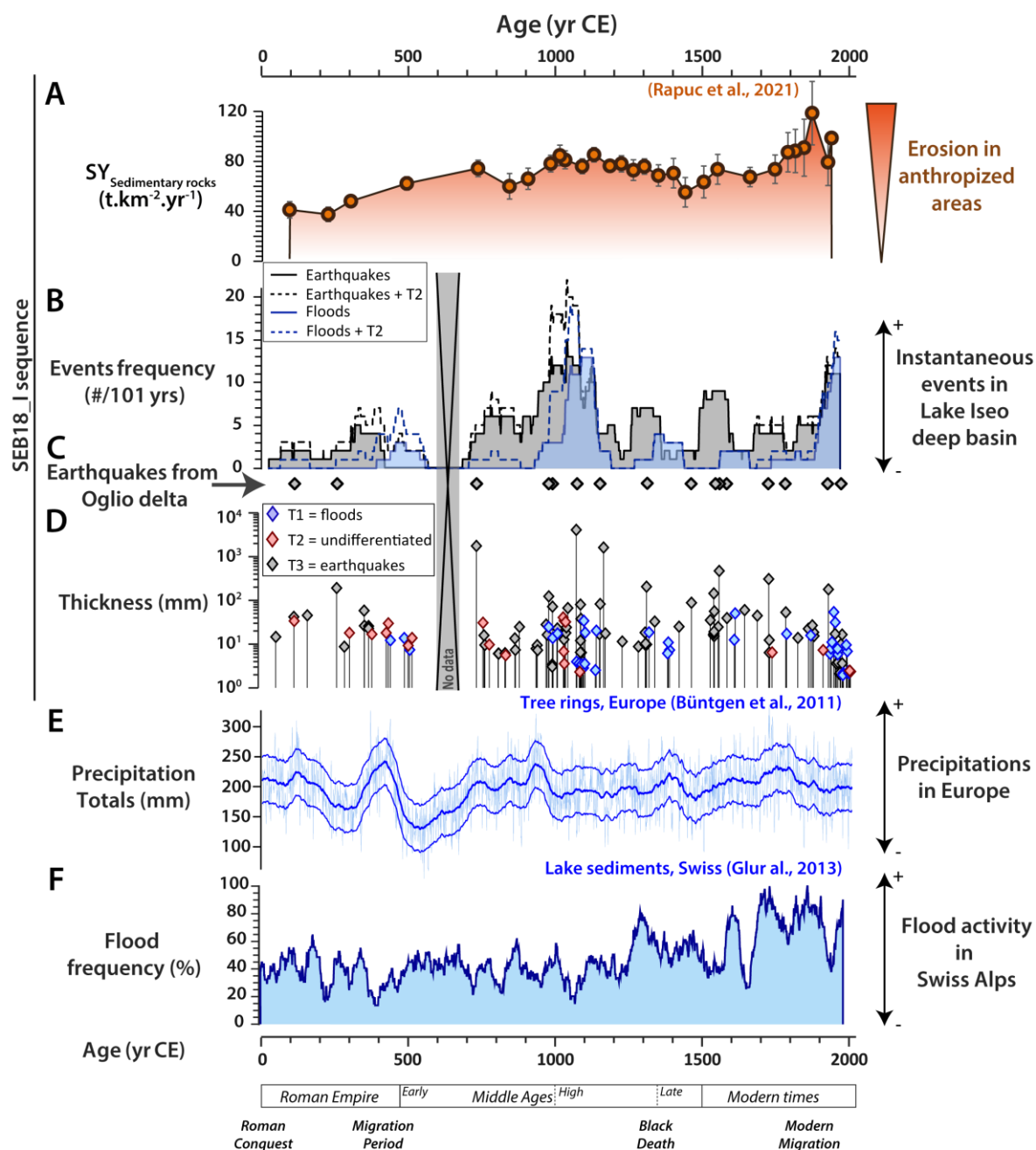
Figure 7 - Comparison of the main results obtained on SEB18 sediment sequence with regional climatic information plotted against the age. (A) The sediment yield of the anthropized area of the Iseo watershed (in t.km^{-2}.yr^{-1} ) obtained from Rapuc et al. (2021). The erosion of this area was interpreted as being mainly influenced by human activities. (B) SEB18 flood and earthquake frequency obtained from ages of Type 1 and Type 3 layers, respectively, Type 1 and 2, and Type 3 and 2 sums are plotted in dotted lines. (C) Type 3 layers with a detrital composition. (D) Thickness of each kind of layer. (E) Reconstructed AMJ precipitation totals modified from Büntgen et al. (2011). (F) 50-year moving average of flood events from Swiss lakes, modified from Glur et al. (2013). et al.
