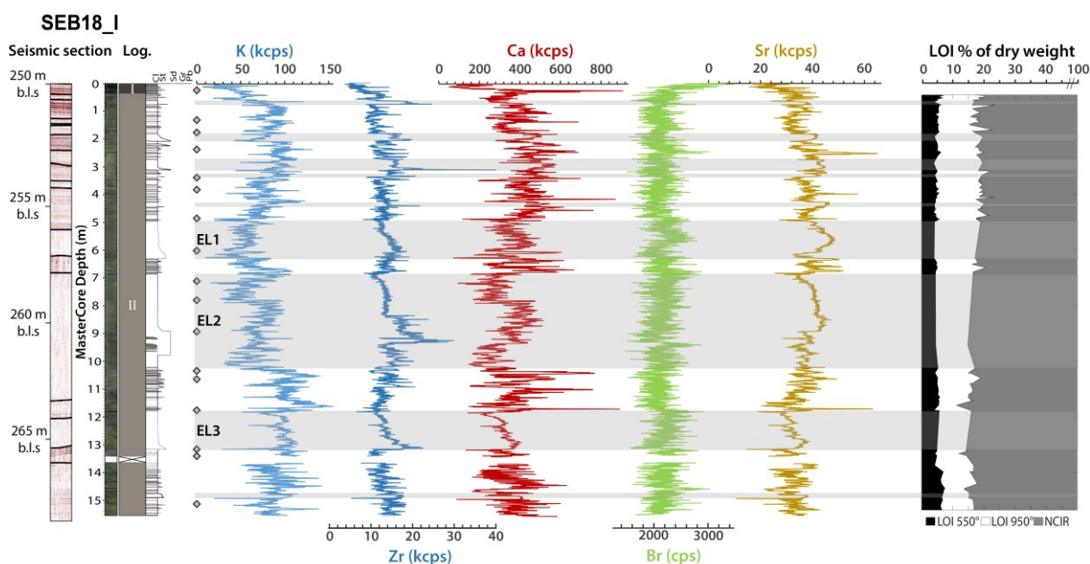
Figure 2 - Sedimentological and geochemical data. A close-up view of the seismic profile (Fig. 1C) section is compared with lithological and geochemical data. A core image of the 15.5 m of the SEB18 sediment sequence and stratigraphic units are associated with the grain-size sensitive lithological column, selected geochemical results (K, Zr, Ca, Br and Sr contents) and loss on ignition (LOI). The depth of the seismic section is expressed in metres below lake surface using a V_p of 1450 \text{ m}\cdot\text{s}^{-1} and is scaled approximately to fit the length of the sediment core. Grey shading represents the thickest graded layers. Grey diamonds represent the junction between the different sections of SEB18 sediment sequence.
