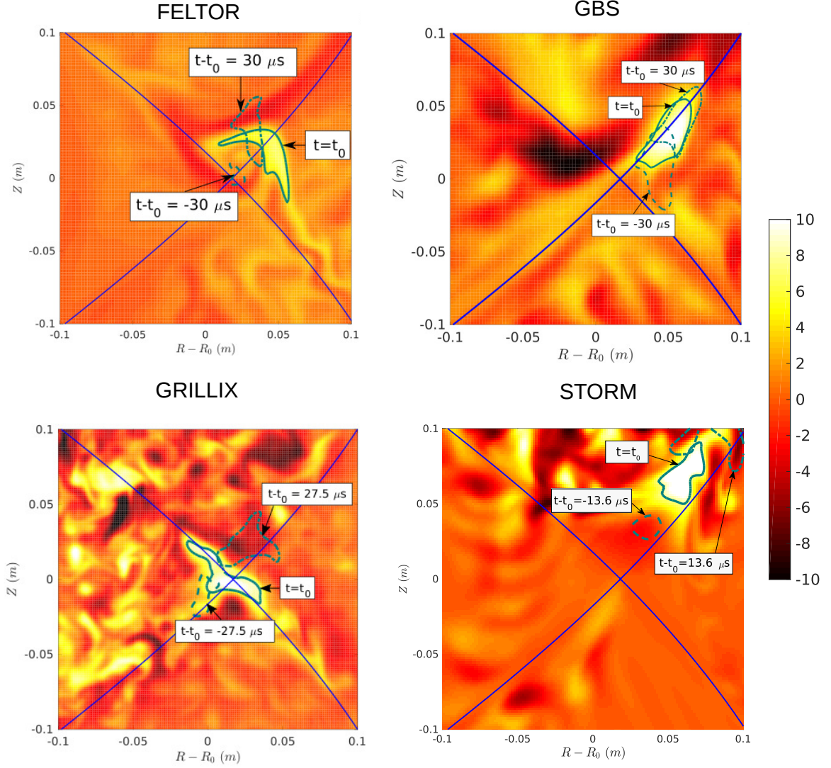
Figure 7: Snapshot of the ion saturation current density fluctuation \delta J_{sat} = J_{sat} - \bar{J}_{sat} ( \text{A/m}^2 ) at a chosen time t_0 , different for each of the codes (zoom around the X-point region). Dashed, solid and dashed-dotted green lines indicate the blob contour at three different time frames, indicated on the figures. The separatrix is represented in blue.
