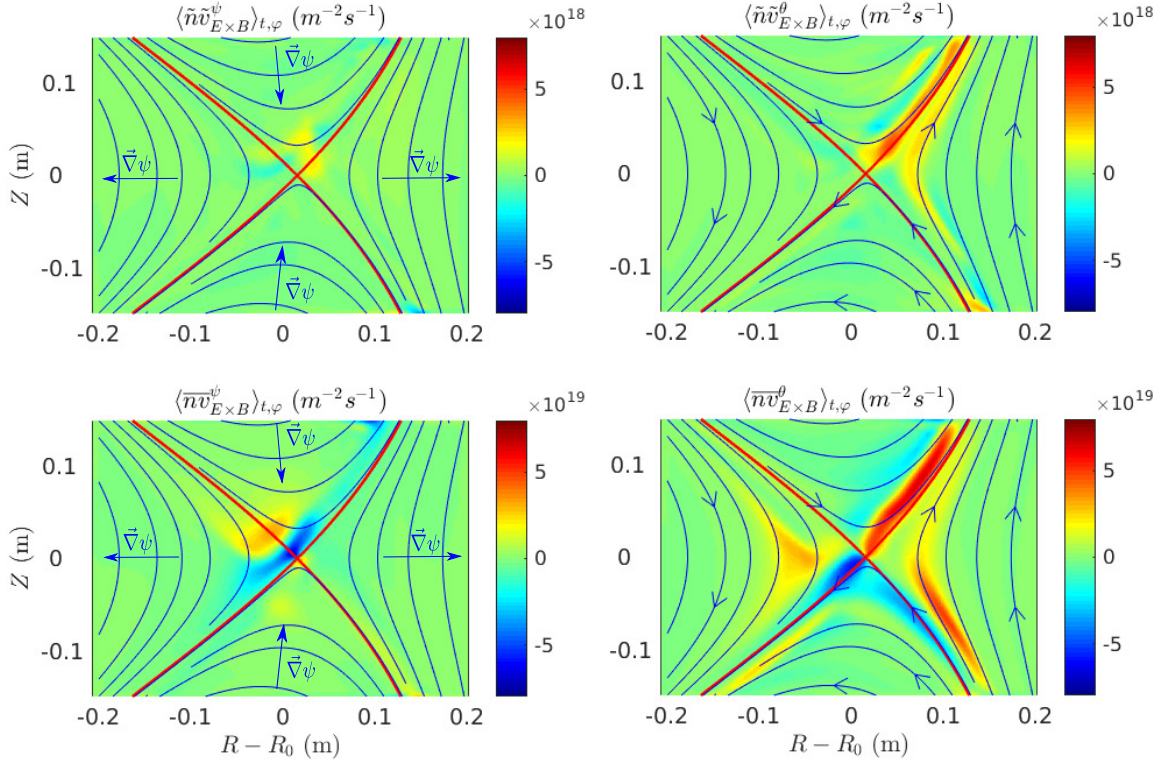
Figure 8: Average in time and toroidal direction of the turbulent and the mean-field components of the E \times B fluxes in the GBS simulation. The E \times B fluxes in the direction \psi across flux surfaces are represented in the left panels, where the arrows indicate the positive \psi direction. The E \times B fluxes in the poloidal direction \theta are represented in the right column, where the arrows indicate the positive \theta direction. The turbulent and the mean-field components are represented in the top and in the bottom row, respectively. Note the difference in the colorbar between top and bottom row.
