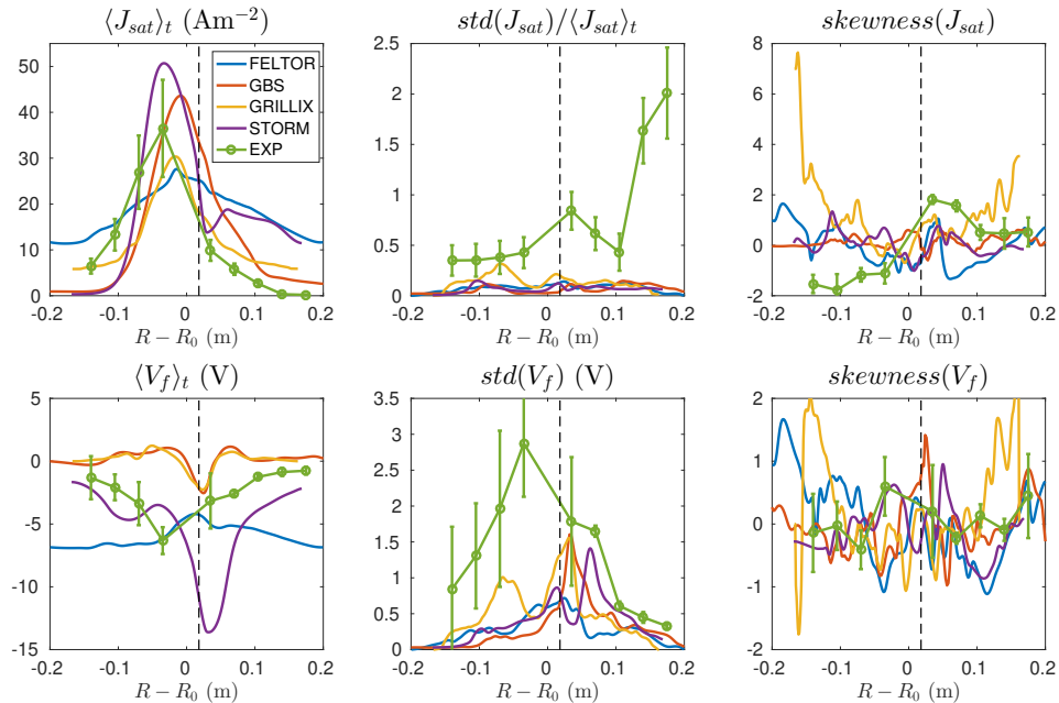
Figure 6: Radial profiles of statistical moments of the ion saturation current density and of floating potential at the midplane ( Z = 0 cm), compared with experimental data from HEX TIP-U. The vertical dashed line indicates the position of the X-point. The evaluation of the experimental errorbars is explained in Section 4.4.
