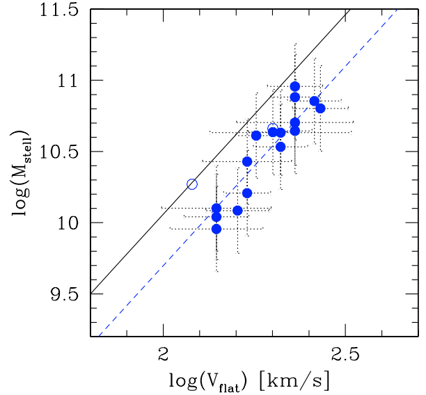
Fig. A.1. Evolution of the stellar-mass TFR in the RD subsample (the two RD+ galaxies are represented with open blue dots). The black line is the local smTFR, while the blue dash-line represents a linear fit to the z \sim 0.6 smTFR.
