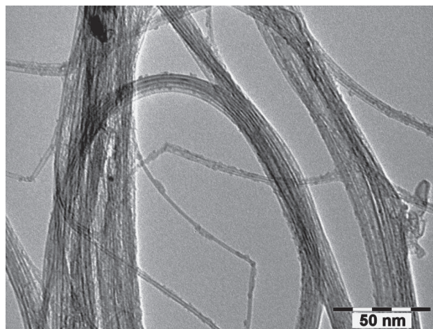
Fig. 1 Typical image of the DWNT bundles after catalyst dissolution.
