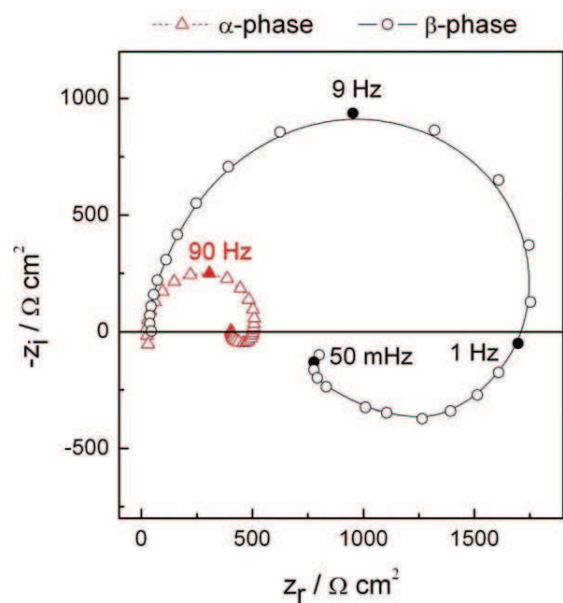
Fig. 6. Nyquist plots of the local electrochemical impedance response of the AZ91 alloy after 2 h immersion in 1 mM \text{Na}_2\text{SO}_4 solution at the corrosion potential. The spectra were recorded close to the electrode centre at various locations over the alloy.
