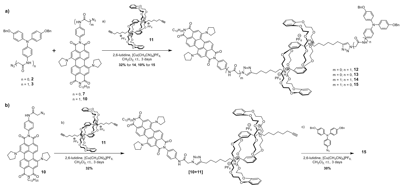
Scheme 3. a) One-pot synthetic route towards unsymmetrical [c2] daisy chain rotaxanes 12-15 ; b) Sequential synthetic route towards unsymmetrical [c2] daisy chain rotaxane 15 .
