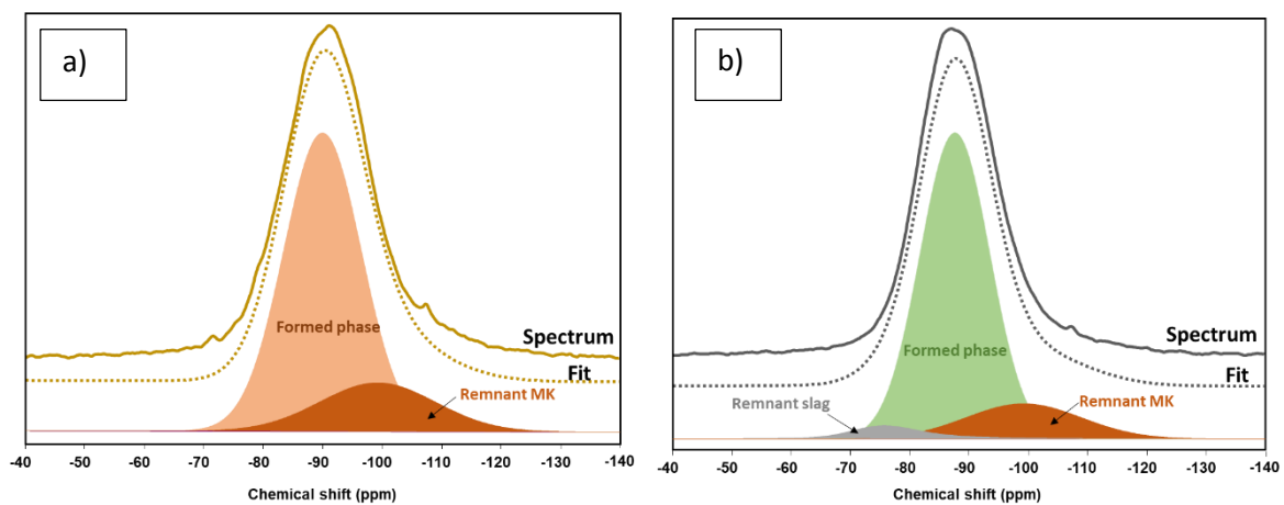
14 15 16 17 18 19 20 21 22 23 24 25 26 27 28 29 30 31 32 33 34 35 36 37 38 39 40 41 42 43 44 45 Figure 5. Decompositions of the ^{29}Si MAS NMR spectra of a) activated metakaolin MK21 and b) activated metakolin-slag MKS21 at 28 days using method 1
