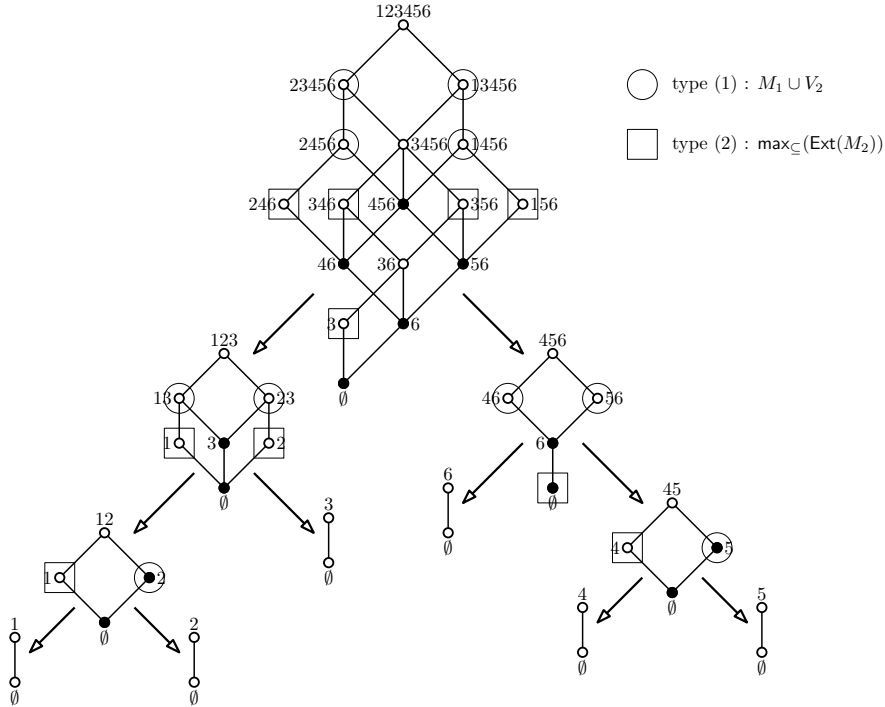
Figure 20: Recursive computation of \mathcal{M} using a decomposition by acyclic splits.
