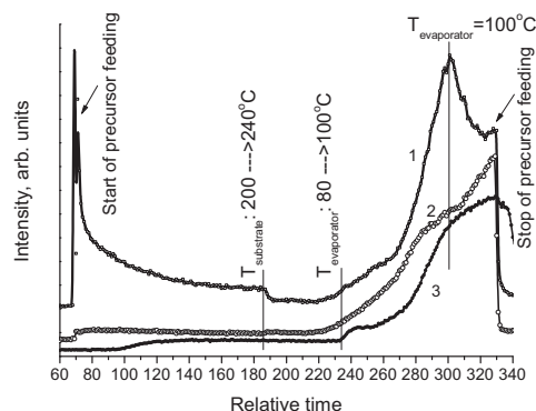
Fig. 1: Time dependence of intensity of ion peaks characterized the gas phase composition upon choosing the temperature conditions: 1- m/z 66 (fragmentary ion from [CpCuPEt 3 ] + ), 2- [Cp 2 ] + , 3- [PEt 3 ] + .
