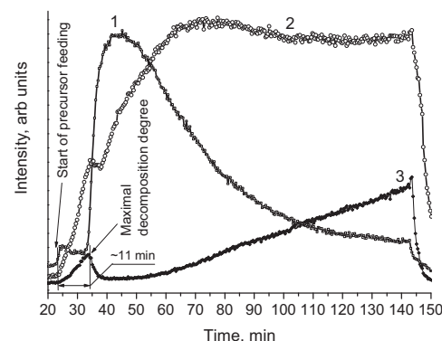
Fig. 2: Time dependence of intensity of ion peaks characterized the gas phase composition upon CVD: 1- [Cp 2 ] + , 2- [PEt 3 ] + , 3- m/z 181 (fragmentary ion from [CpCuPEt 3 ] + ).
