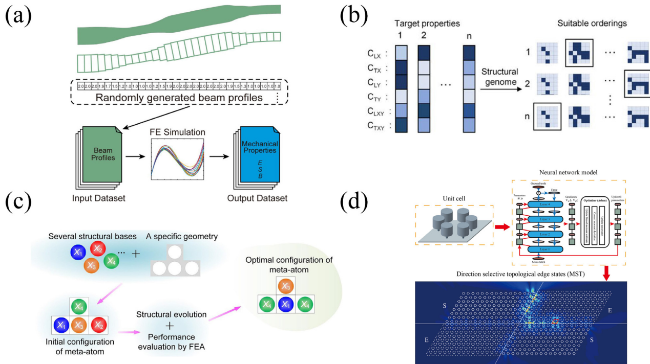
Figure 7: Applying neural networks for elastic metamaterials design.
