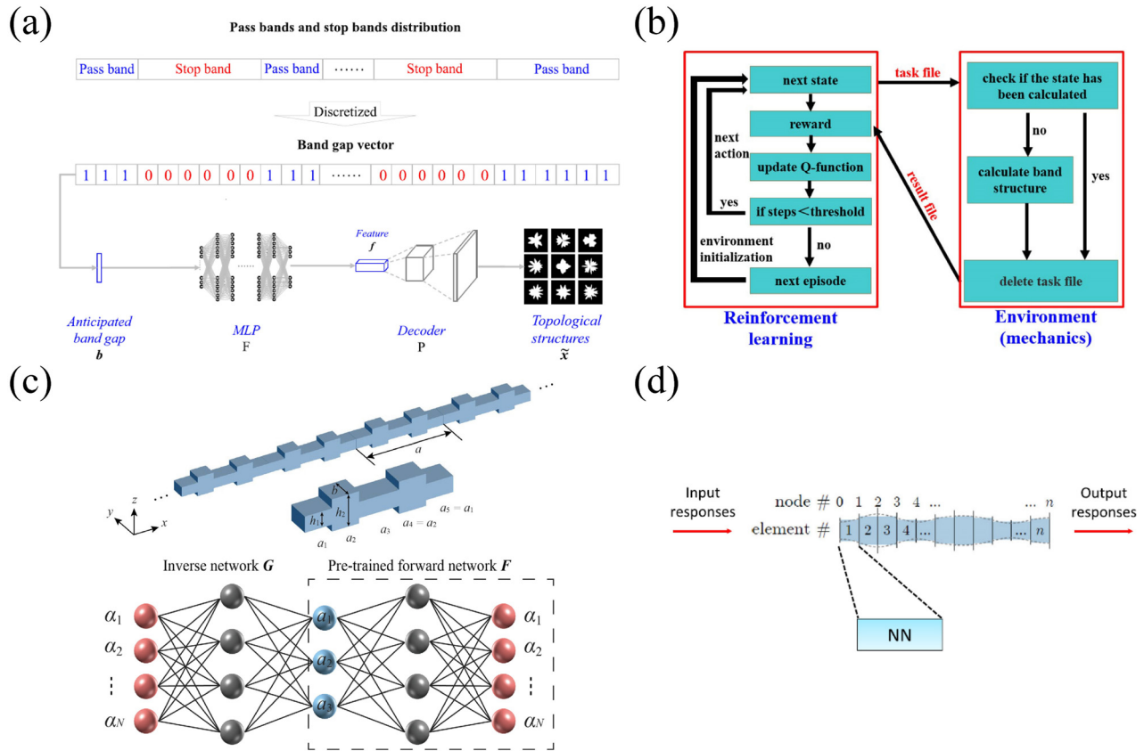
Figure 8: Elastic metamaterials design enabled by advanced neural network model and reinforcement learning.
