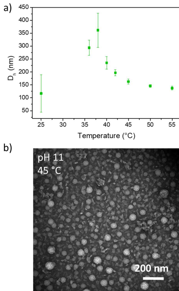
Figure 9. a) Multi-angle DLS analysis: evolution of the estimated hydrodynamic diameter as a function of temperature from 25 to 55 °C of a PVAm 10 -b-PNIPAM 50 @pH11 aqueous solution at 0.01% w/v. Measurements were carried at each temperature with a return to ambient temperature in between. b) TEM image of PVAm 10 -b-PNIPAM 50 @pH11 deposited on a copper-carbon grid from a solution at 0.1% w/v at 45 °C
