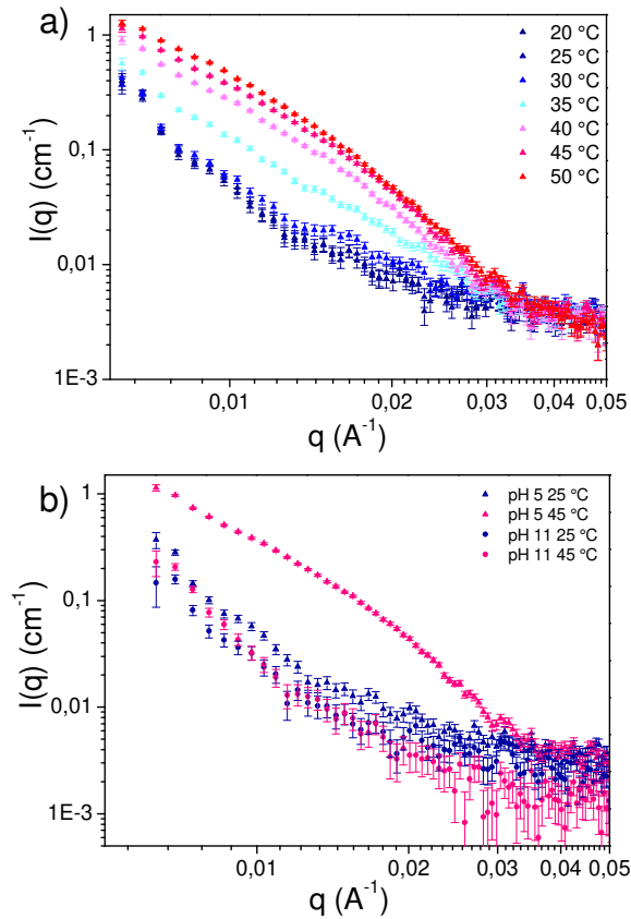
Figure 13. Scattering curves of a) PVAm 10 - b -PNIPAM 50 at pH 5 as a function of temperature from 20 °C to 50 °C and of b) PVAm 10 - b -PNIPAM 50 at pH5 (▲) and pH11 (●) at 25 °C (blue) and 45 °C (pink).
