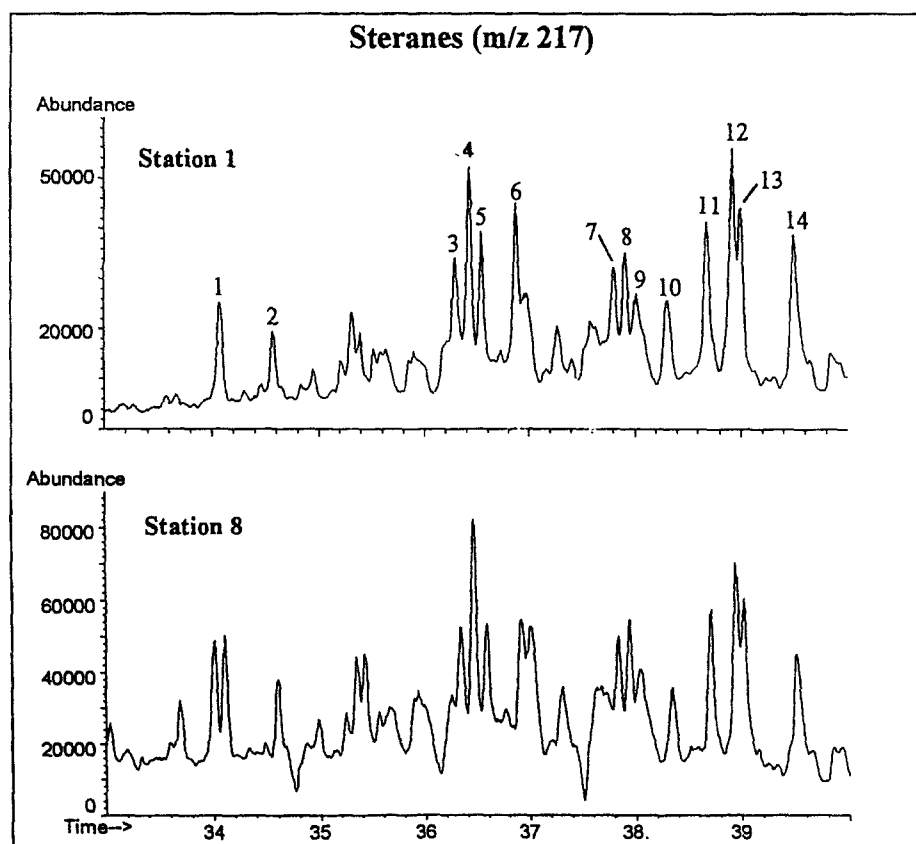
Fig. 3 Chromatograms of tricyclic terpanes, tetracyclic terpanes and pentacyclic terpanes (hopanes) (m/z=191), steranes and diasteranes (m/z 217) (stations 1 and 8; 2-7 cm layer).
