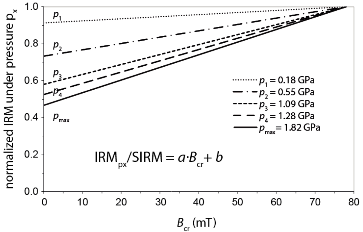
Figure 3. Empirical dependency of normalized isothermal remanent magnetization ( IRM_{p_x}/SIRM ) under hydrostatic pressure p_x ( x=1,2,3\dots ) versus remanent coercivity B_{cr} for Fe-Ni-bearing ordinary chondrites. This graph gives a predictive model, which can be used to determine the degree of pressure demagnetization of Fe-Ni-bearing samples for given pressure and B_{cr} values with 5% accuracy.
