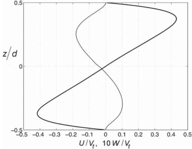
FIG. 1. Averaged velocity profiles in the vertical midplane. Bold line: streamwise velocity; thin line: crosswise velocity. Lengths are normalized by the pipe diameter d and velocities are normalized by V_t = (Atgd)^{1/2} .
