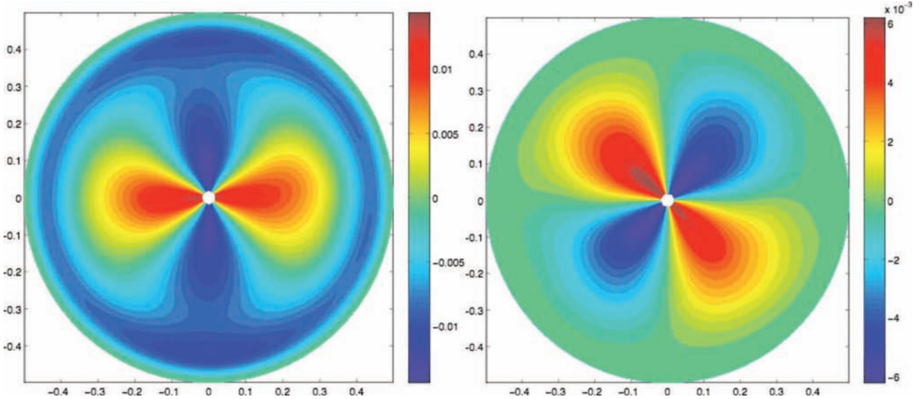
FIG. 4. (Color online) Map of the secondary anisotropy \langle v_r^2 \rangle - \langle v_\theta^2 \rangle (left) and cross correlation \langle v_r v_\theta \rangle (right), both normalized by V_t^2 .
