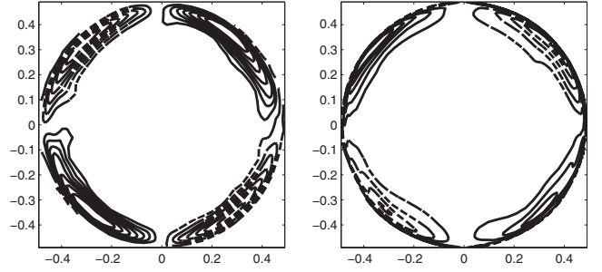
FIG. 3. Map of the turbulent term \mathcal{R} (left) and baroclinic term \mathcal{B} (right) in Eq. (1), both normalized by (V_t/d)^2 . The contour levels of \mathcal{R} range from -0.342 to 0.342 with a step of 0.049 , while those of \mathcal{B} range from -0.085 to 0.085 with a step of 0.015 . Solid (dashed) lines denote positive (negative) values. The zero level has been removed for clarity.
