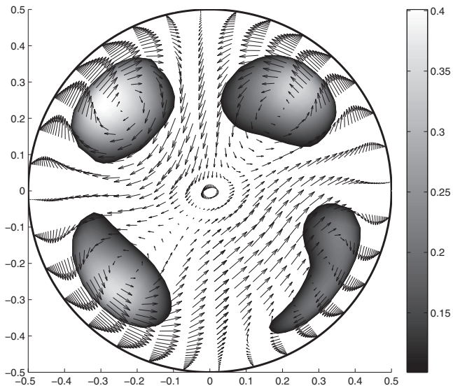
FIG. 2. Mean secondary flow and streamwise vortices identified by the magnitude of the swirling strength ( \lambda_{ci} criterion). The normalization is similar to that of Fig. 1.
