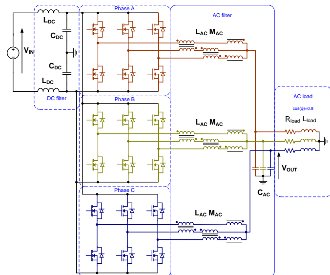
Fig. 5. 3-Phase inverter with 3-interleaving coupled levels
