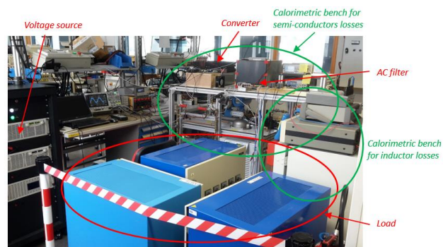
Fig. 20. Experimental setup with the test benches
