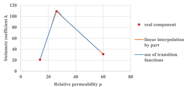
Fig. 7. Steinmetz coefficient k variation with the relative permeability
