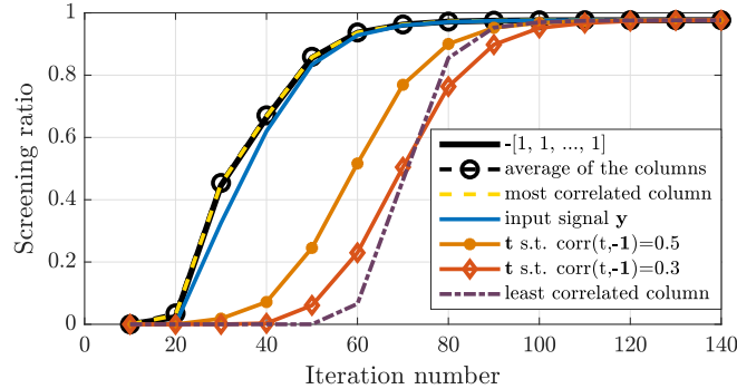
Fig. 2. Screening performance with different choices for the translation vector \mathbf{t} on a NNLS problem with the NIPS papers dataset (described in Section 5.2).
