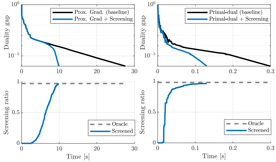
Fig. 4. Convergence and screening ratio for the BVLS hyperspectral experiment. Speedups of 2.79 and 2.30 are achieved respectively for the projected gradient (left) and primal-dual (right) solvers.
