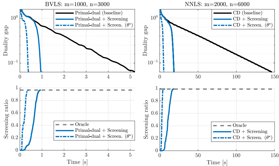
Fig. 3. Duality gap convergence (top) and screening ratio (bottom) through time for the simulation setups described in Tables 1 and 2. Left: BVLS problem with primal-dual solver. Right: NNLS problem with coordinate descent solver. The dashed curves correspond to the screening approach artificially informed with an optimal dual point ( \theta^* ), which reaches a speedup of 12.8 (left) and 27.8 (right).
