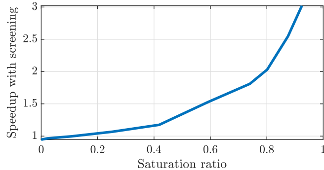
Fig. 1. Speedup w.r.t. saturation ratio for a BVLS problem of size m = 4000 , n = 2000 , solved with projected gradient descent. The matrix \mathbf{A} \in \mathbb{R}^{m \times n} and vector \mathbf{y} \in \mathbb{R}^m have been generated according to a_{ij} \sim \mathcal{N}(0, 1) and y_i \sim \mathcal{N}(0, 1) . The saturation ratio is controlled by varying the size of the box b[-\mathbf{1}, \mathbf{1}] .
