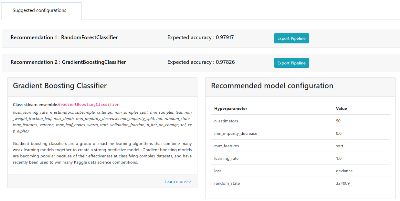
Fig. 7 AutoML overview.
