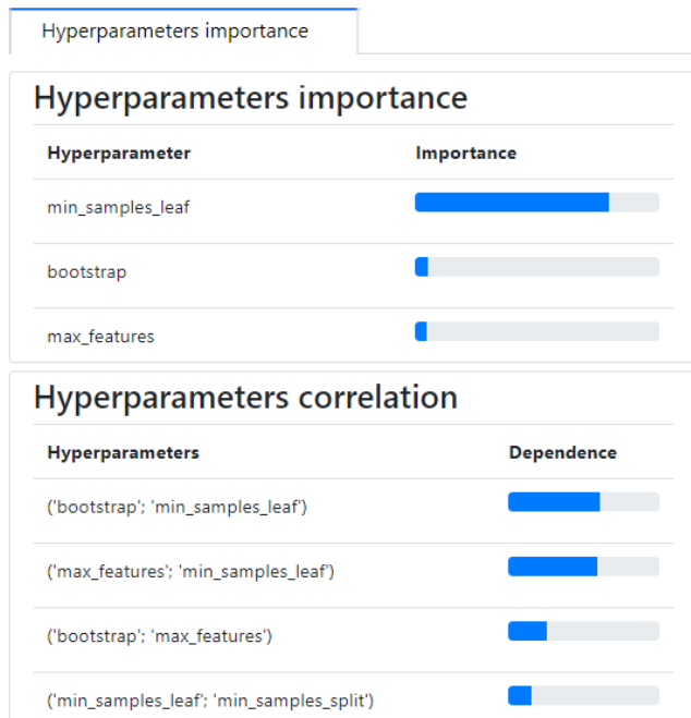
Fig. 10 Refinement-level view.
