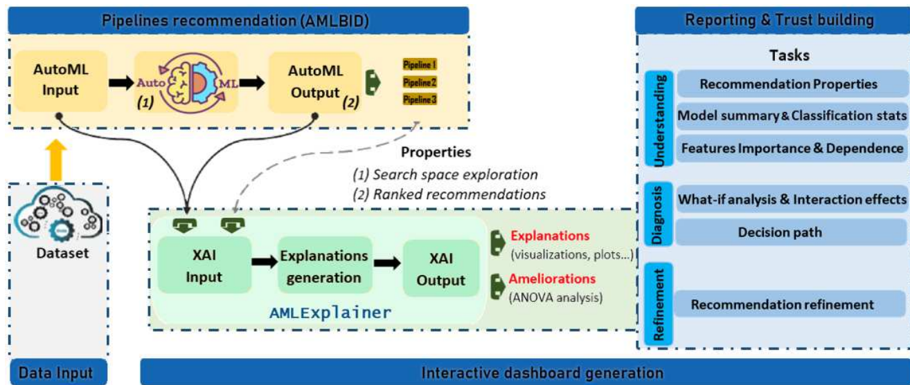
Fig. 3 The global architecture of the proposed white-box AutoML (AMLBD and AMLExplainer).
