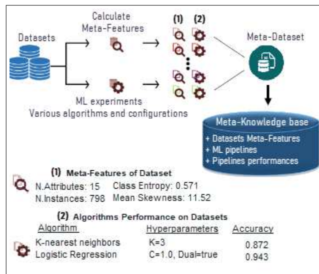
Fig. 4 Learning phase workflow.
