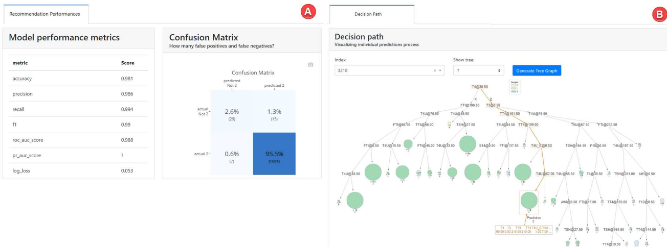
Fig. 8 Recommendation-level view.
