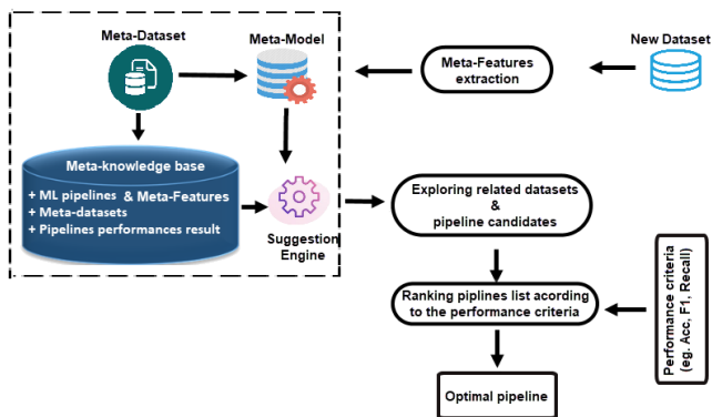
Fig. 5 Recommending phase workflow.
