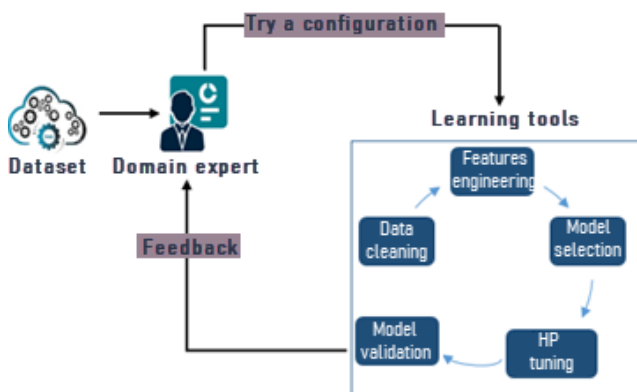
Fig. 1 The ML configuration tuning process.
