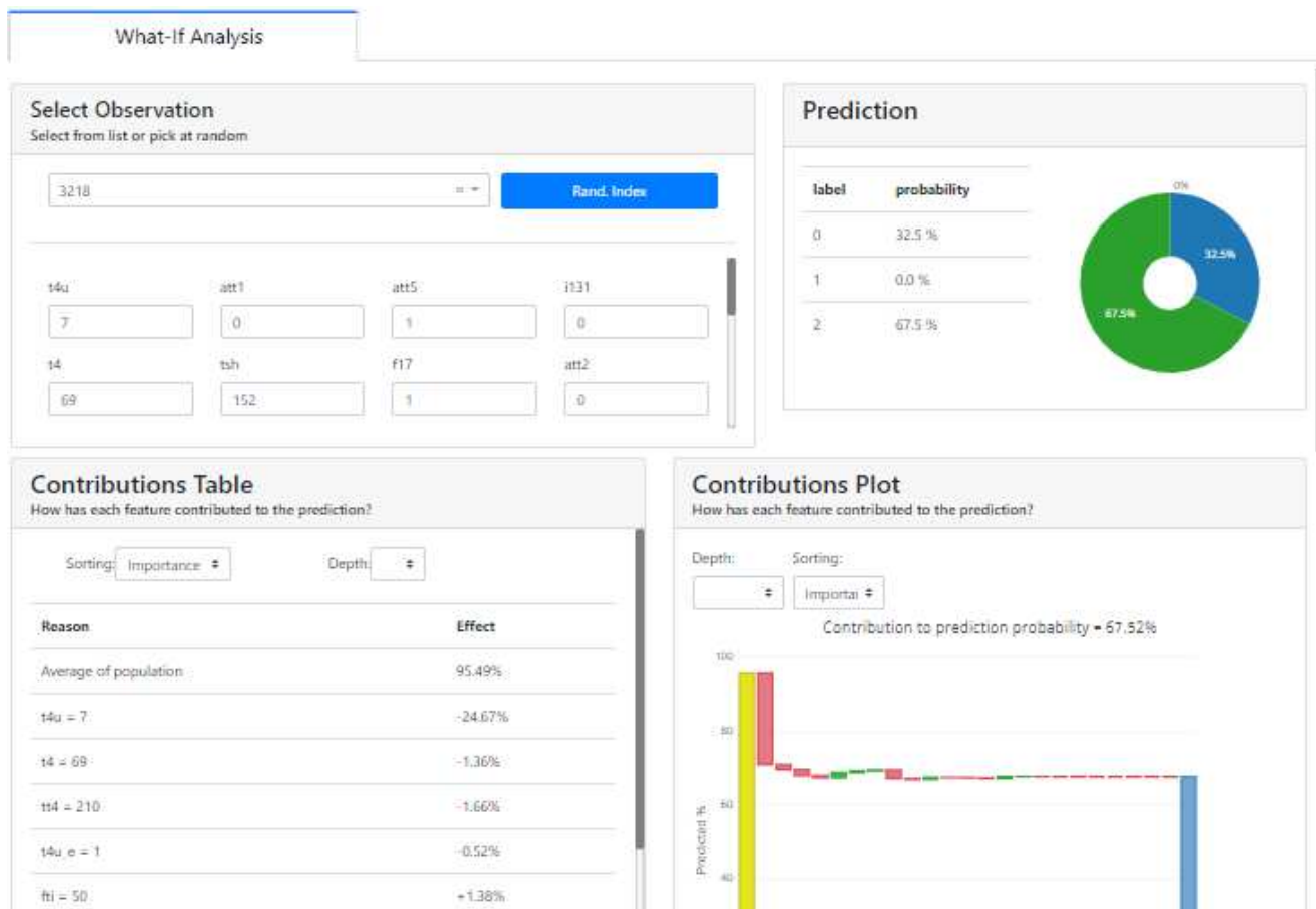
Fig. 9 What-if analysis-level view.
