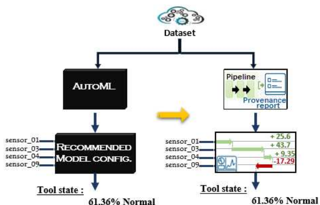
Fig. 2 “Black-box” model recommendation and prediction to “White box” model with explanations.
