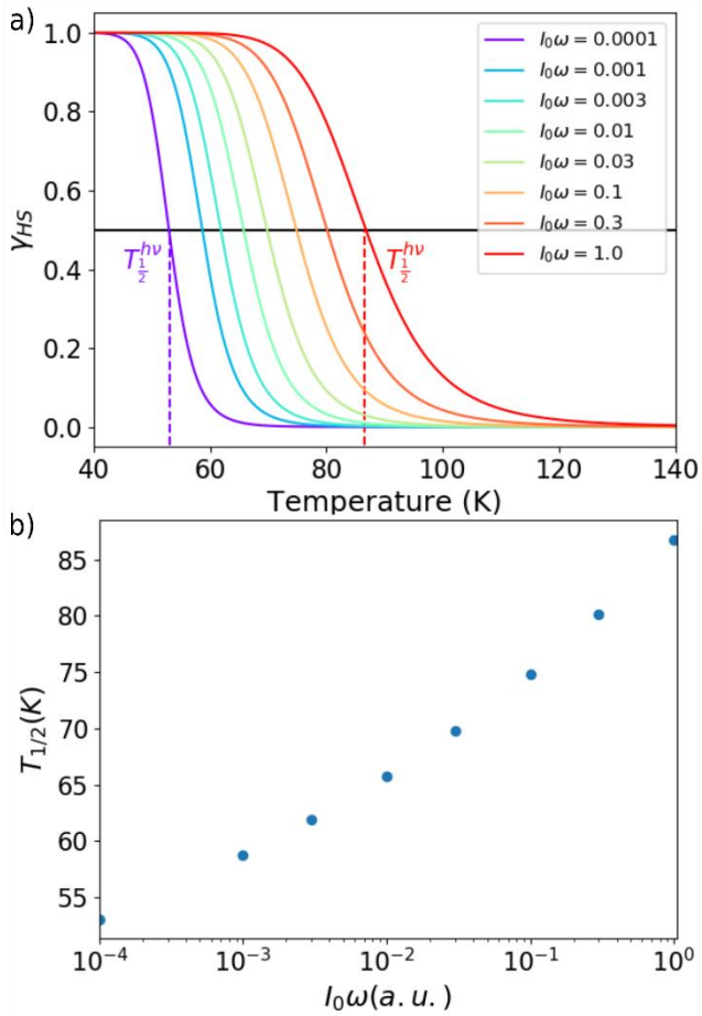
Fig. 4. a) Calculated temperature dependence of the photo-stationary HS fraction. b) Evolution of T_{1/2}^{hv} with I_0\omega .
