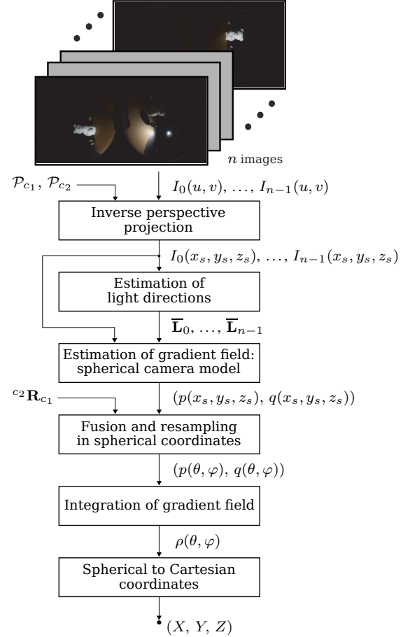
Fig. 2. Flowchart of the proposed photometric stereo algorithm, which takes n dual-fisheye images as input.
