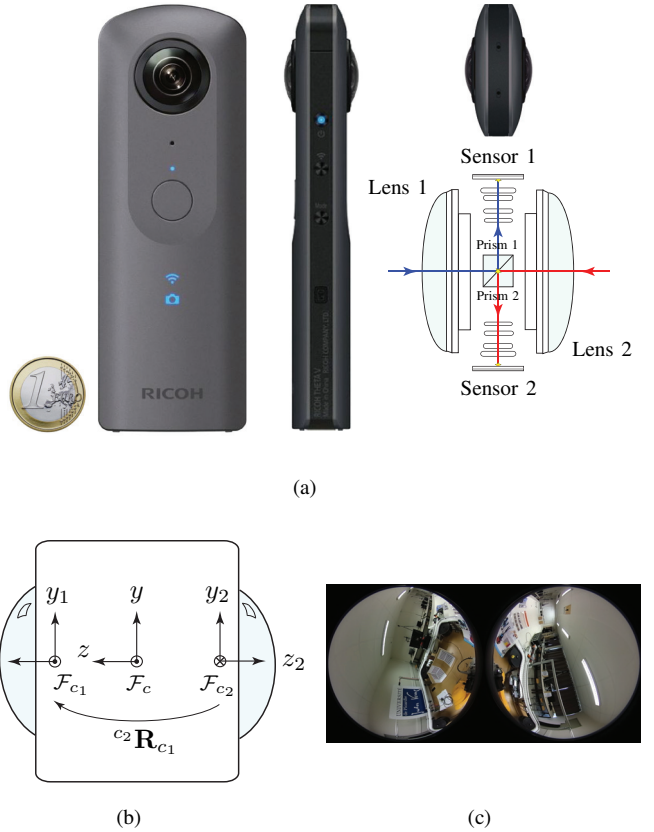
Fig. 1. (a) Front, side and top view of a twin-fisheye camera, the Ricoh Theta V (image courtesy of Ricoh), and schematic of the optical system with the two fisheye lenses, prisms and CMOS sensors; (b) \mathcal{F}_c is the camera frame, and \mathcal{F}_{c_1}, \mathcal{F}_{c_2} , the reference frames associated to the two fisheye lenses (top view); (c) Example of dual-fisheye image taken by the Ricoh Theta V: the left and right sub-images correspond to the two fisheye lenses.
