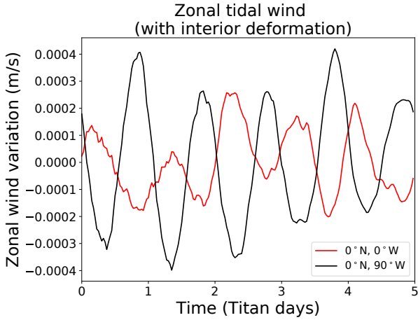
Fig. 8. Component of zonal tidal winds at 35 m above the surface computed at latitude 0°N and longitude 0°W (red) or 90°W (black). The lines correspond to the difference between simulations with tides and without tides. Thermal tides were not included in these simulations.
