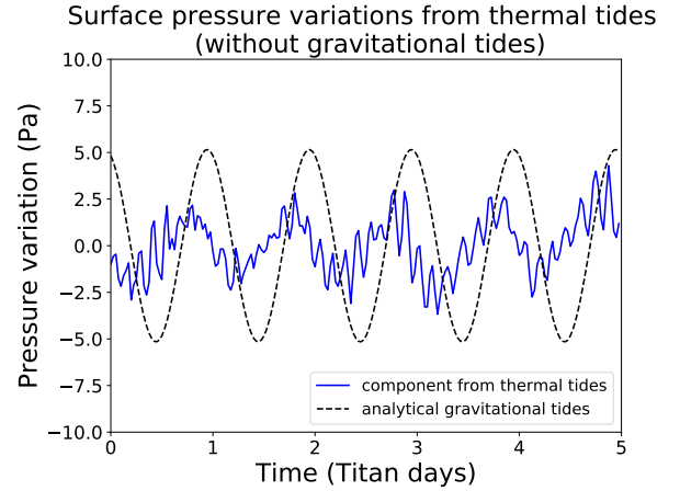
Fig. 7. Pressure variations caused by thermal tides at longitude 0^\circ and latitude 0^\circ\text{N} computed with the Titan IPSL GCM. The analytical pressure variation from gravitational tides with interior deformation is shown with a black dashed line.
