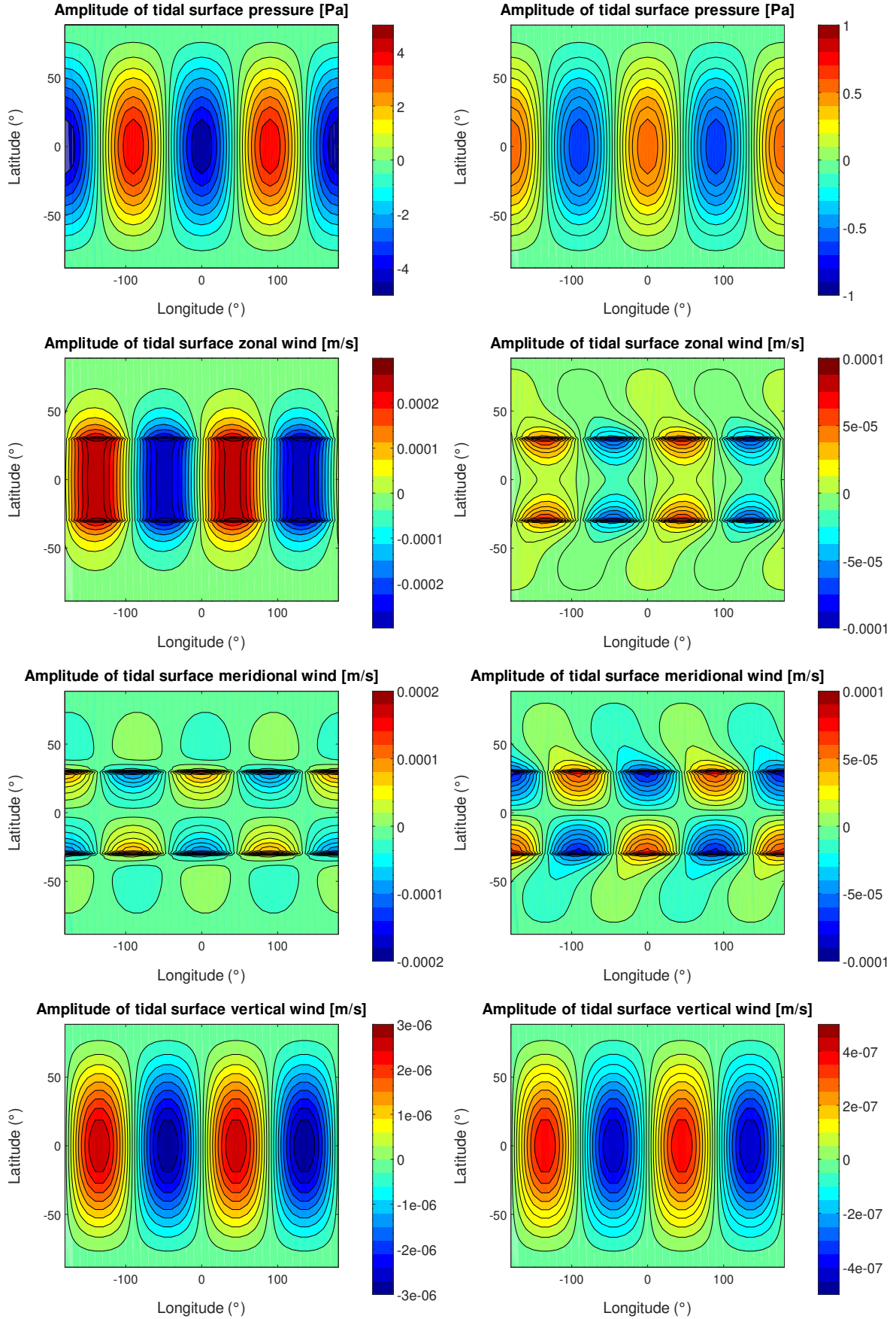
Fig. 5. Tidal surface pressure and tidal zonal, meridional, and vertical surface winds as functions of longitude and latitude at t = 0 for the eastward wave (left) and the westward wave (right). Analytical calculation including interior deformation with 1 + \Re(k_2 - h_2) = 0.08 and \Im(k_2 - h_2) = 0.01 .
