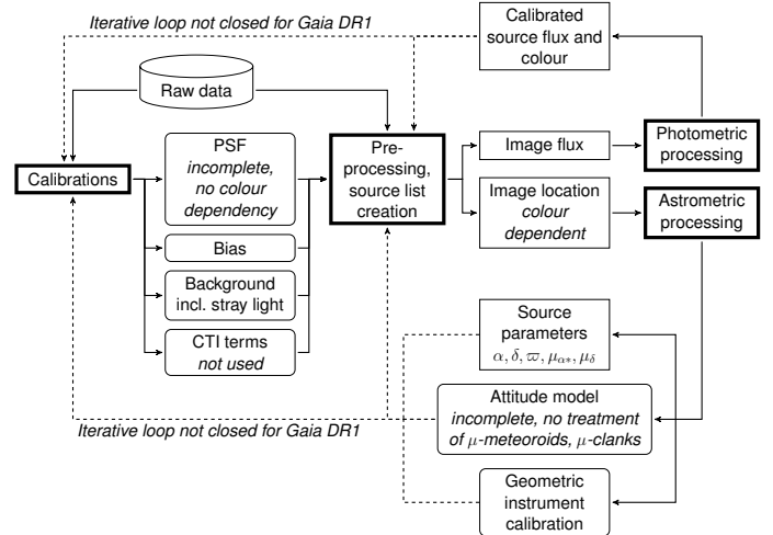
Fig. 10. The DPAC data processing flow as used for Gaia DR1 in schematic and simplified form. Thick lined boxes show processing steps, rounded boxes represent calibrations derived during the processing, while thin-lined boxes show processing outputs. The solid lines indicate the processing flow as realised for Gaia DR1, while the dashed lines indicate processing flows that were not implemented for Gaia DR1. The remarks in italics highlight important shortcomings in the Gaia DR1 processing.
