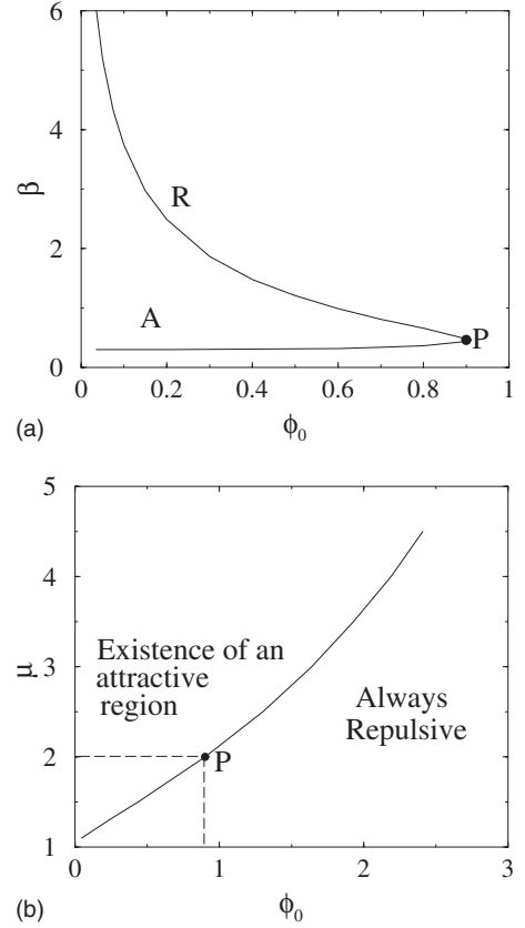
FIG. 4. Investigation of attractiveness in the phase space of the parameters of the problem. (a) (\beta-\phi_0) plane for \mu=2 . R stands for repulsion and A for attraction. Point P ( \beta \approx 0.465 , \phi_0 \approx 0.9 ) corresponds to the minimum equal to zero of the pressure curve represented in Fig. 3(b) (b) (\mu-\phi_0) plane. Long-dashed lines locate point P in this plane.
