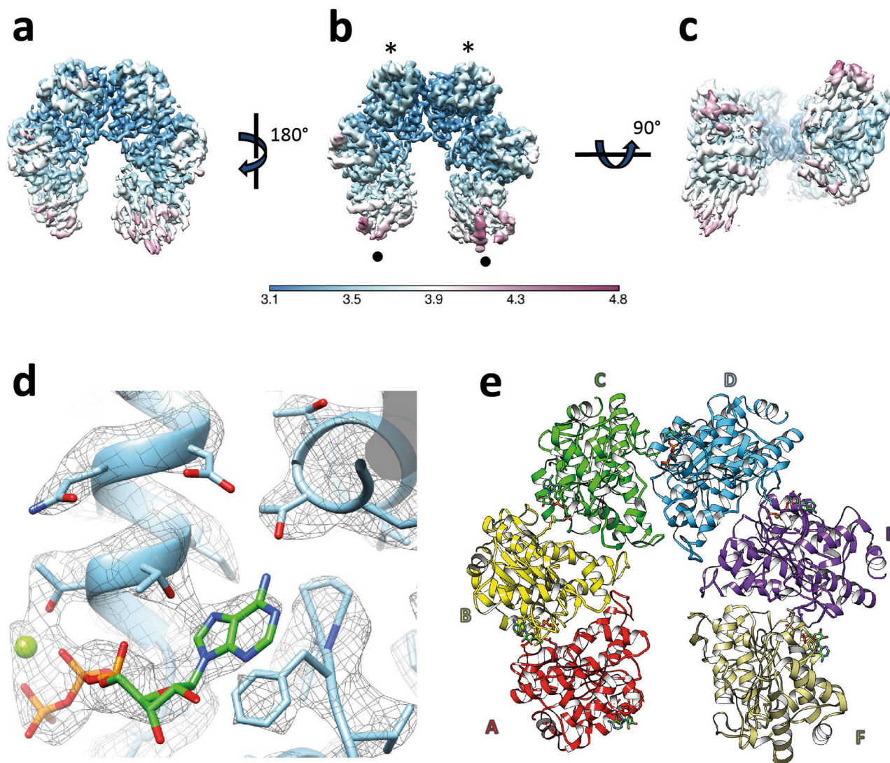
Fig. 1 Single-particle cryo-EM structure of the M. tuberculosis Rho complex. a–c The 3.3 Å cryo-map of M_{tb} Rho colored according to local resolution from highest (dark blue) to lowest resolution (dark purple). The M_{tb} Rho is composed of six subunits adopting an open corkscrew conformation. When observed from top ( a ) or down ( b ) views, M_{tb} Rho displays a U-like shape where the two subunits at the gap are the less well-resolved (black dots) while the innermost subunits (black stars) are the best resolved. The side view c highlights the shift between the two gap subunits that results from the corkscrew arrangement of the M_{tb} Rho ring. The first ~220 N-terminal residues of each protomer are not resolved. d Close-up view of the ATP binding site at the C/D interface. The M_{tb} Rho atomic model and cryo-EM map are superimposed. The ATP phosphates are in orange, sugar in green, oxygen groups in red and adenine base in green/blue. The catalytic Mg^{2+} ion is shown as a green sphere. e Refined PDB structure of M_{tb} Rho. The subunits are labeled from A to F in clockwise order, observed from the CTD face of the M_{tb} Rho hexamer as in B.
