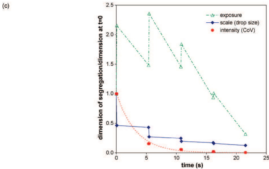
Fig. 7 – (a) Progress of an injected additive as drops break up and dissolve over time. Drop break-up is restricted to the impeller zone, and dissolution is restricted to the bulk. (b) Snapshots of the sample volume over the dissolution process. Dissolution steps are from the top row to the bottom row, and the corresponding values of time, drop size, CoV, and exposure are given in table. (c) Comparison of the scale, intensity, and rate of change of segregation as they change over time, all normalized with the initial values in step 1.
