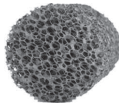
Fig. 2. Characteristics of \beta -SiC foam studied.
