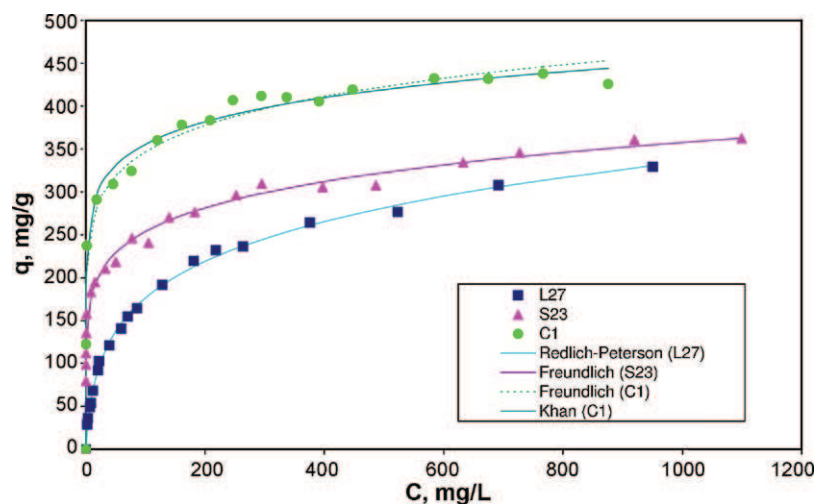
Fig. 3. Adsorption isotherms of levodopa on L27, S23 and C1 carbons at 25 °C. q is the amount of adsorbed compound at equilibrium per unit amount of adsorbent (mg/g AC ); C is the concentration of adsorbate in aqueous phase at equilibrium (mg/L).
