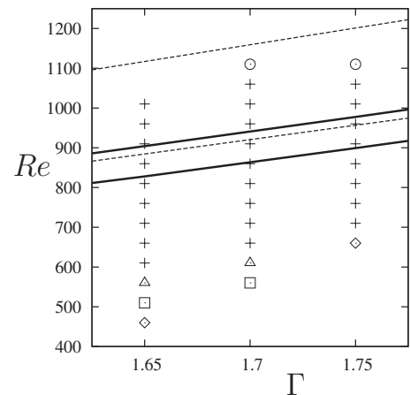
FIG. 3. Bifurcation diagram at low Re . The markers show experimental results. + : Detached bubble; \circ : corner bubble; \times : attached bubble; \triangle : detached+corner bubble; \diamond : detached bubble with inner structure; \square : corner bubble with inner structure. The full lines are bifurcation curves obtained from simulations. The lower curve is the creation of a detached bubble while the top curve is the corner crossing bifurcation to a corner bubble. The dashed lines are the corresponding experimental curves found by Spohn et al. (Ref. 8).
