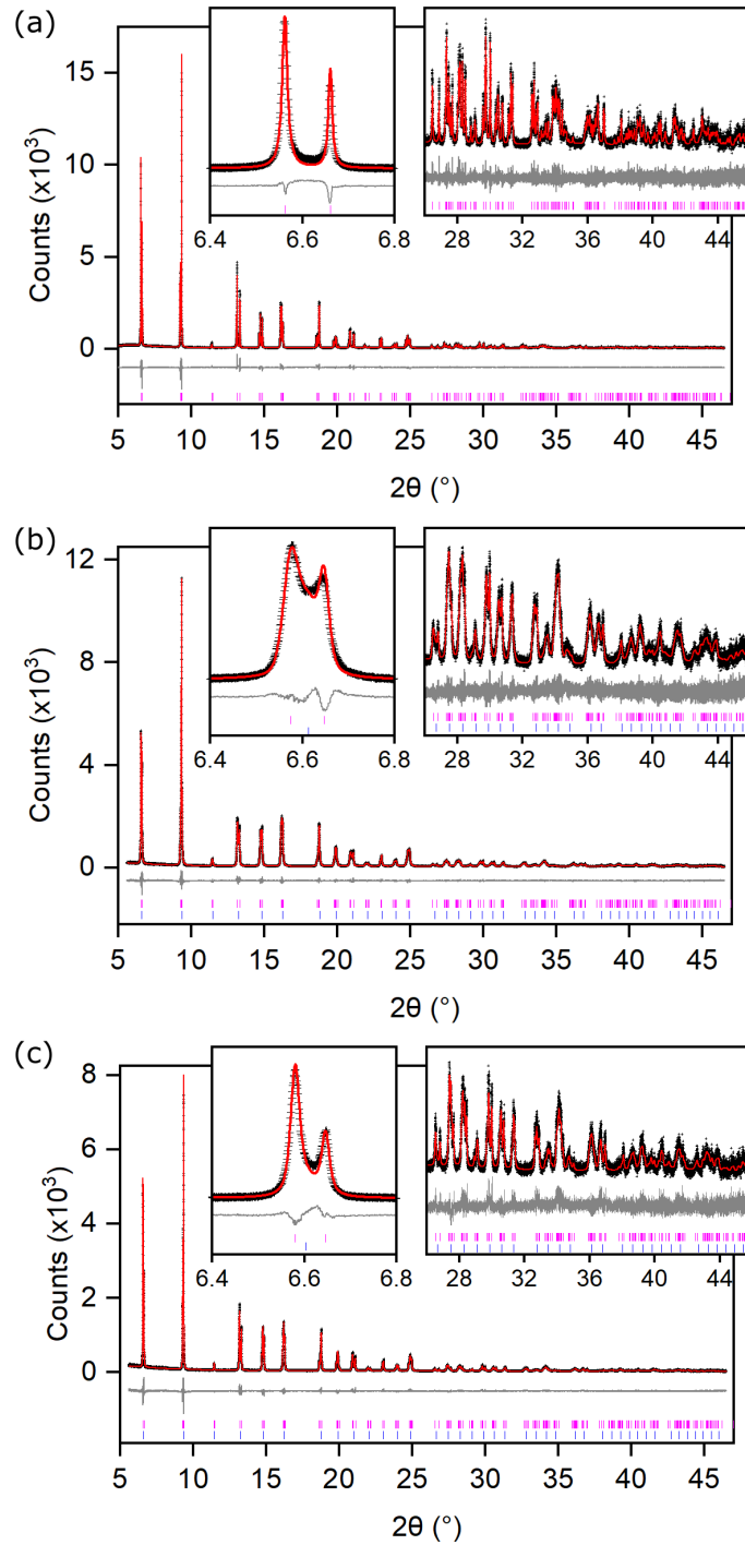
Figure 5: Rietveld refinements against SPD data for (a) KNN fitted to a single Amm 2 perovskite, (b, c) KNNTa and KNNTa-prec fitted to a two-phase mixture of Amm 2 and Pm \bar{3} m perovskites. Magnified views of the (011)/(100) peaks and high-angle regions are shown as insets.
