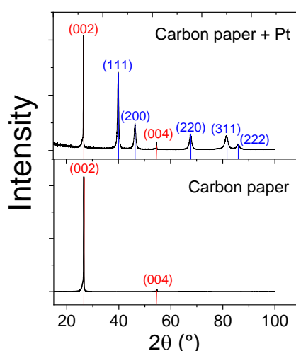
Figure 2. XRD spectra of carbon paper (bare CP) and Pt@CP.
