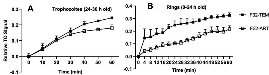
Fig. 5. Impact of ART (1 \mu\text{M} ) on Plasmodium cellular homeostasis on trophozoite (24–36 h old) (A) and ring (0–24 h post invasion) (B) stages. ART treatment had significantly ( p < 0.05 ) more impact on F32-TEM than F32-ART in the first 4 min at the ring stages while there was no statistical difference at the trophozoite stage. The results are triplicates from 3 independent experiments and p -values obtained after a regression analysis of each graph at 95% confidence interval.
