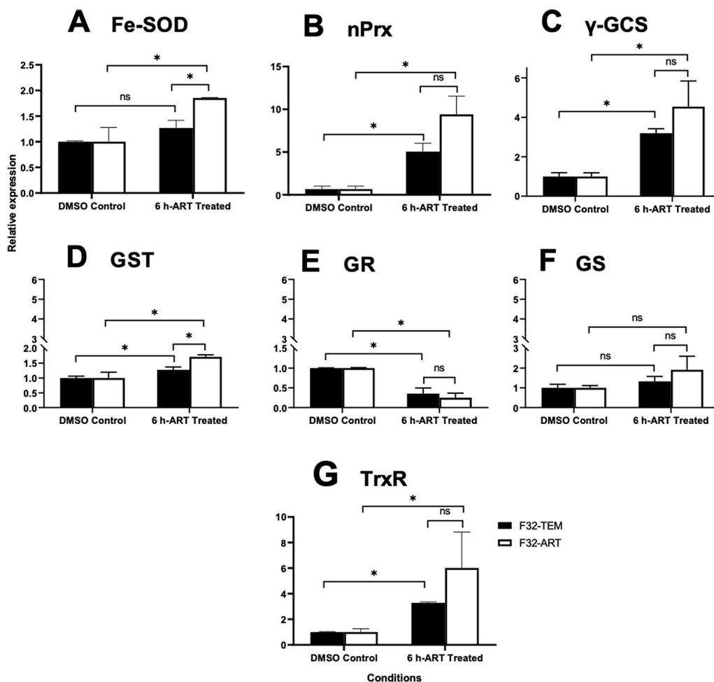
Fig. 8. Impact of ART treatment on the transcriptional profiles of antioxidants. Relative expression of antioxidant enzymes (A: Fe-SOD = Iron-superoxide dismutase, B: nPrx = Peroxiredoxin, C: \gamma -GCS = \gamma -glutamylcysteine synthetase, D: GST = Glutathione-S-transferase, E: GR = Glutathione reductase, F: GS = Glutathione synthetase and G: TrxR = Thioredoxin reductase) in F32-ART (ART-resistant) and F32-TEM (ART-sensitive) strains treated with artemisinin (at 3 \mu M during 6 h) comparatively to the DMSO control (corresponding to the value 1). The results are duplicates from three independent biological samples (performed with 0–24 h old rings). The values were analyzed using t -test. * p < 0.005.
