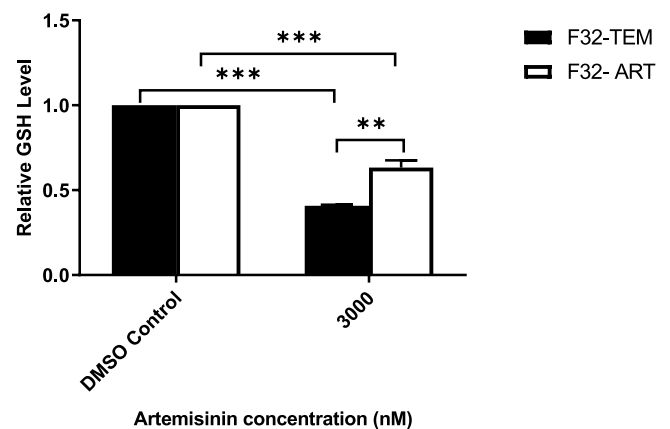
Fig. 10. Impact of artemisinin exposure (3 \mu M, after a 4 h treatment) on Plasmodium falciparum reduced glutathione (GSH) at the ring stage (0–24 h post invasion). F32-TEM showed significantly ( p < 0.05 ) higher susceptibility to GSH depletion than F32-ART under ART treatment. These results are triplicates from one experiment. The fold depletion in GSH was 0.41 \pm 0.00 for F32-TEM and 0.63 \pm 0.04 for F32-ART, compared to untreated control. ** = p < 0.01 and *** = p < 0.001 .
