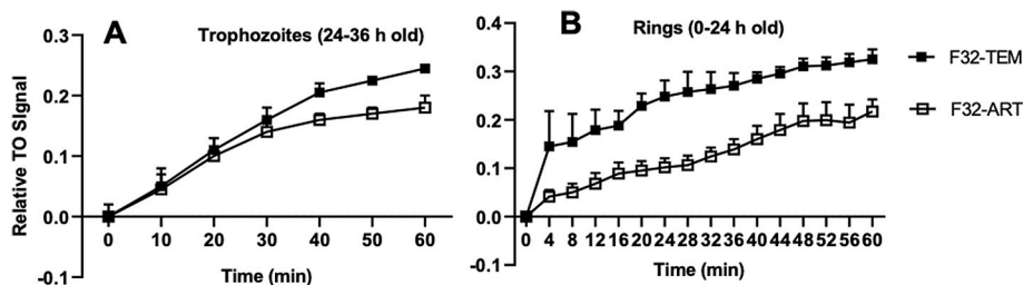
Fig. 5. Impact of ART (1 \mu\text{M} ) on Plasmodium cellular homeostasis on trophozoite (24–36 h old) (A) and ring (0–24 h post invasion) (B) stages. ART treatment had significantly ( p < 0.05 ) more impact on F32-TEM than F32-ART in the first 4 min at the ring stages while there was no statistical difference at the trophozoite stage. The results are triplicates from 3 independent experiments and p -values obtained after a regression analysis of each graph at 95% confidence interval.
