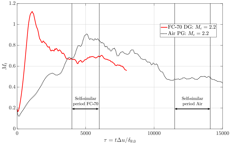
FIGURE 13. Temporal evolution of the turbulent Mach number M_t .
