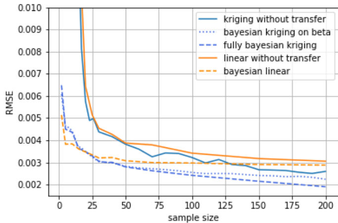
Figure 1: Evolution of the RMSE score for varying number of new observation used to fit the model.
