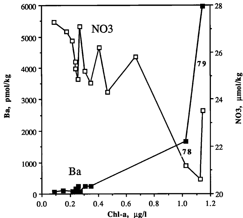
Fig. 6. Particulate barium (solid squares, pmol kg -1 ) and nitrate (open squares, μmol kg -1 ) versus Chl- a (μg L -1 ) in the surface waters (<50 m).
